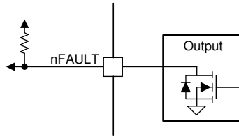
Figure 7-46. nFAULT Pin
