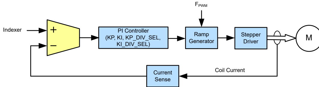
Figure 7-17. Silent step block diagram
