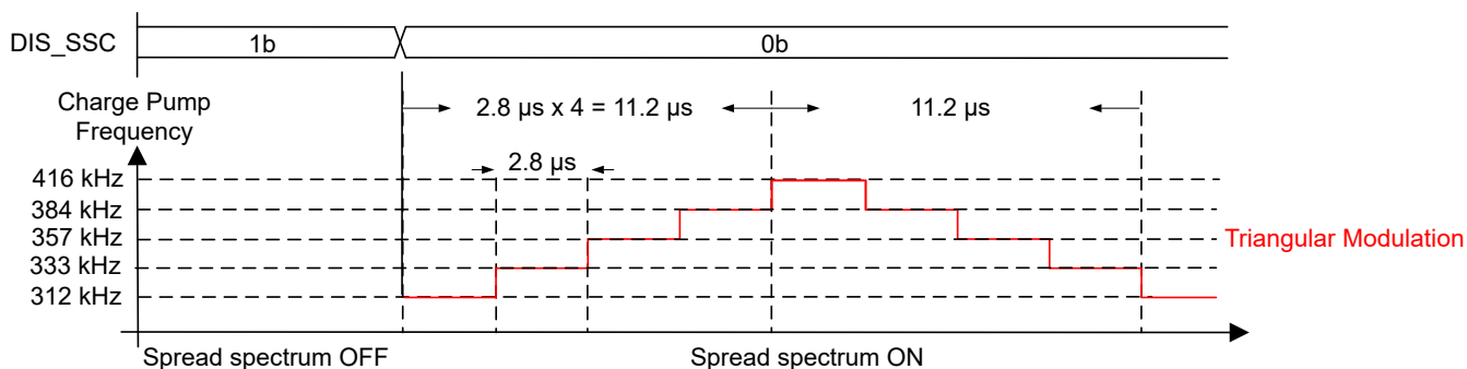
Figure 7-38. Triangular Spread Spectrum of Charge Pump Clock
