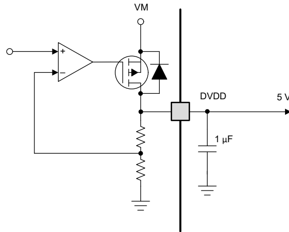
Figure 7-31. Linear Voltage Regulator Block Diagram
