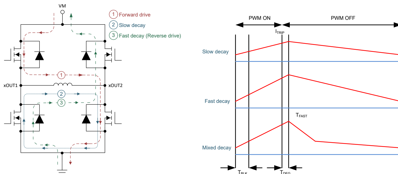
Figure 7-11. Decay Modes
