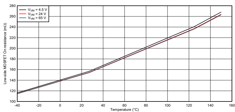
Figure 6-7. Low-side FET on resistance
