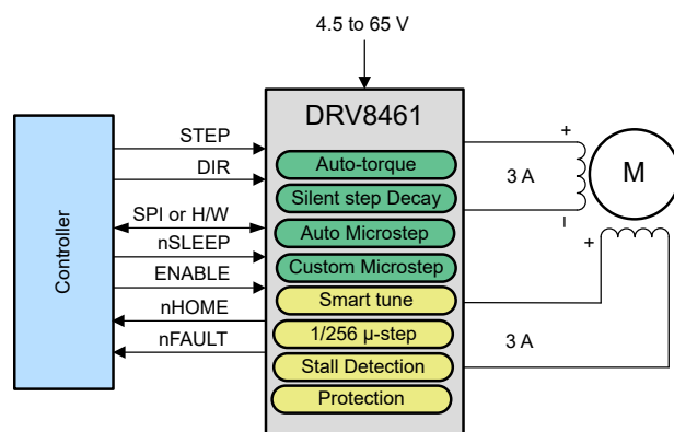
Simplified Schematic
