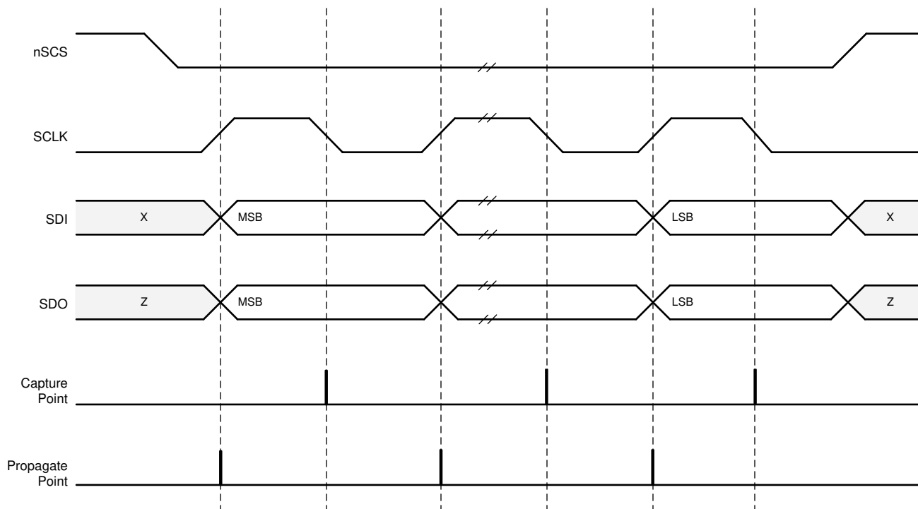
Figure 7-54. SPI Transaction
