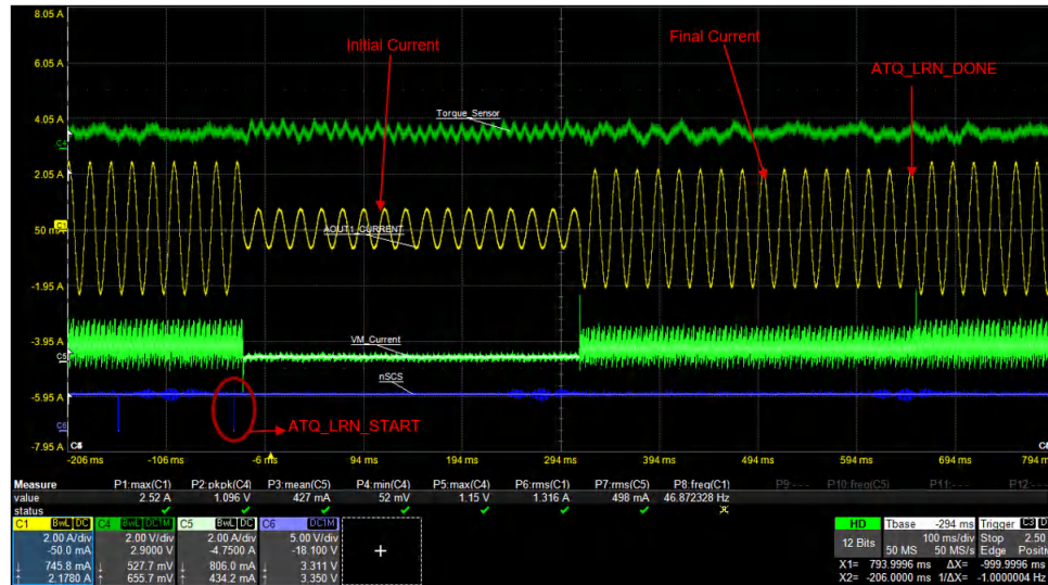
Figure 7-25. Auto-torque learning
