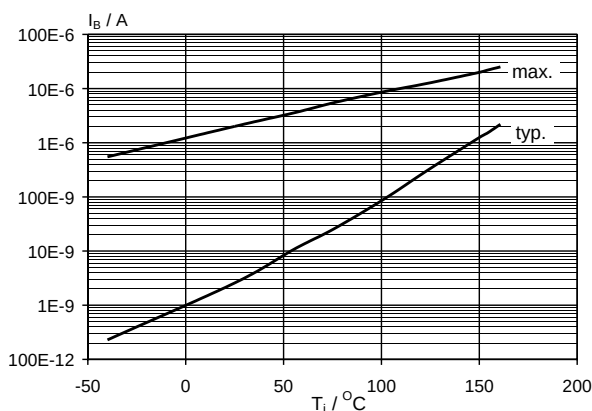
Fig.10. Typical supply quiescent current. I_B = f(T_J) ; condition V_{BG} = 16\text{ V} , V_{IG} = 0\text{ V} , V_{LG} = 0\text{ V}
