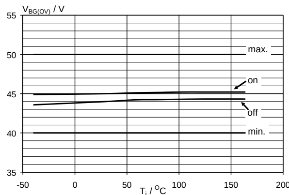
Fig.15. Supply overvoltage thresholds. V_{BG(OV)} = f(T_J) ; conditions V_{IG} = 5\text{ V} ; I_L = 100\text{ mA}
