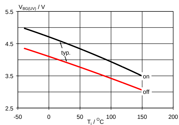
Fig.14. Supply undervoltage thresholds. V_{BG(UV)} = f(T_J) ; conditions V_{IG} = 5\text{ V} ; V_{BL} \leq 2\text{ V}
