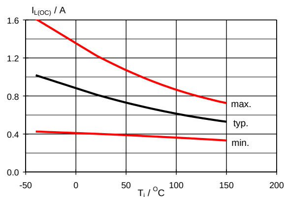
Fig.13. Low load current detection threshold. I_{L(OC)} = f(T_J) ; conditions V_{IG} = 5\text{ V} ; V_{BG} \geq 9\text{ V}
