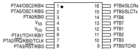
16-PIN ASSIGNMENT MC68HC908QL3 TSSOP
