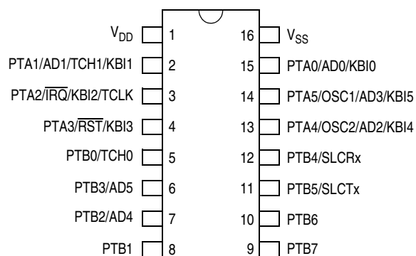
16-PIN ASSIGNMENT MC68HC908QL4 AND MC68HC908QL2 SOIC
