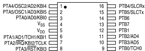
16-PIN ASSIGNMENT MC68HC908QL4 AND MC68HC908QL2 TSSOP
