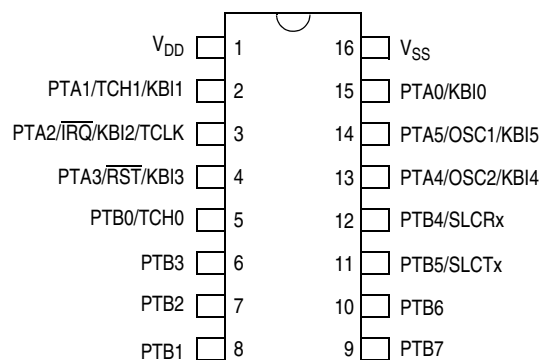
16-PIN ASSIGNMENT MC68HC908QL3 SOIC
