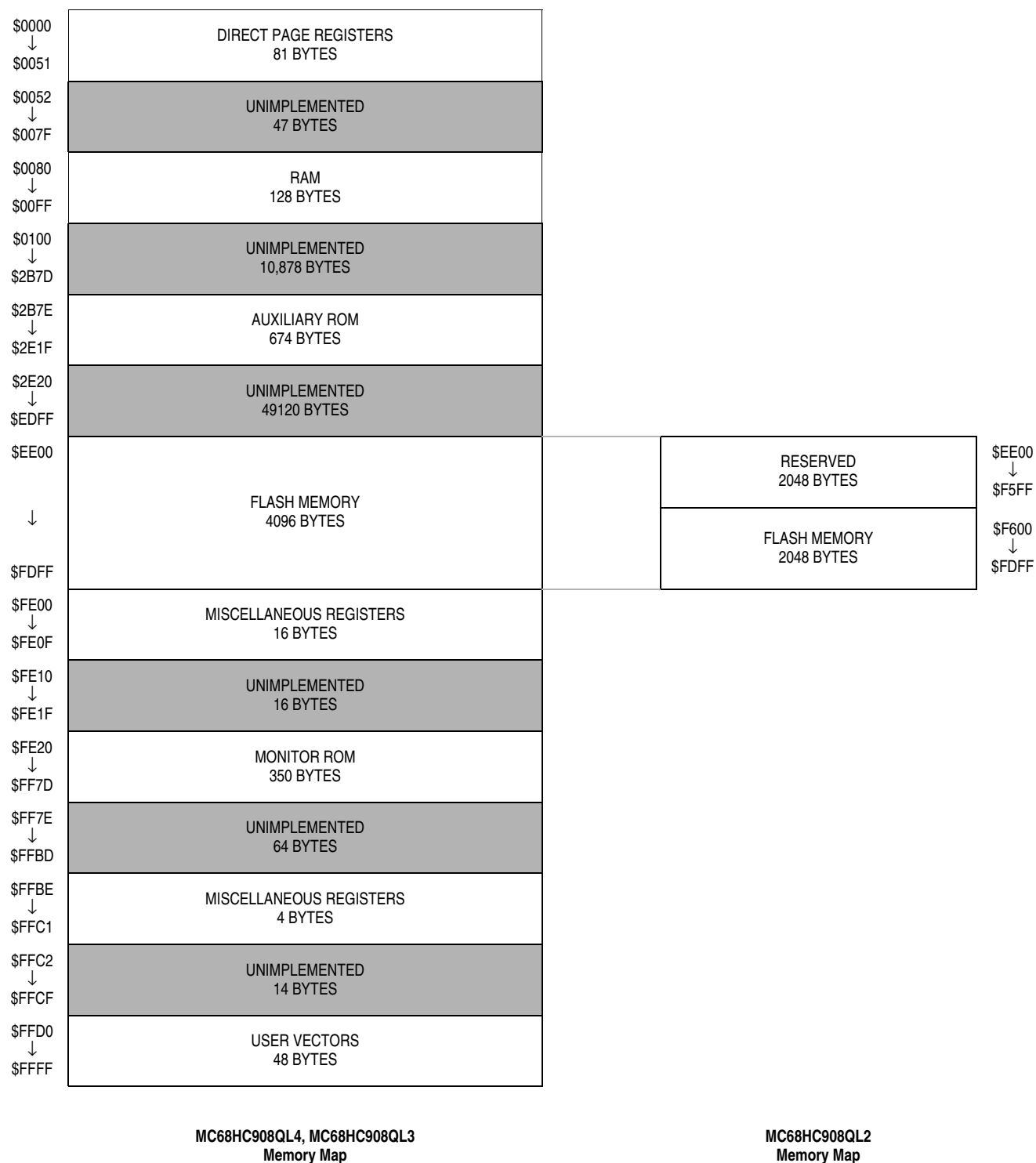
Figure 2-1. Memory Map
