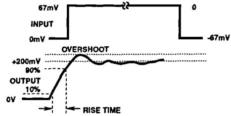
FIGURE 2. TRANSIENT RESPONSE
