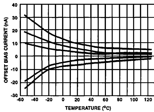
FIGURE 7. OFFSET CURRENT vs TEMPERATURE (5 TYPICAL UNITS FROM 3 LOTS AT V_s = \pm 15V )
