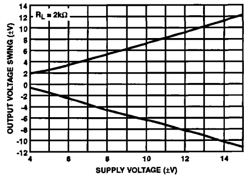
FIGURE 10. OUTPUT VOLTAGE SWING vs SUPPLY VOLTAGE
