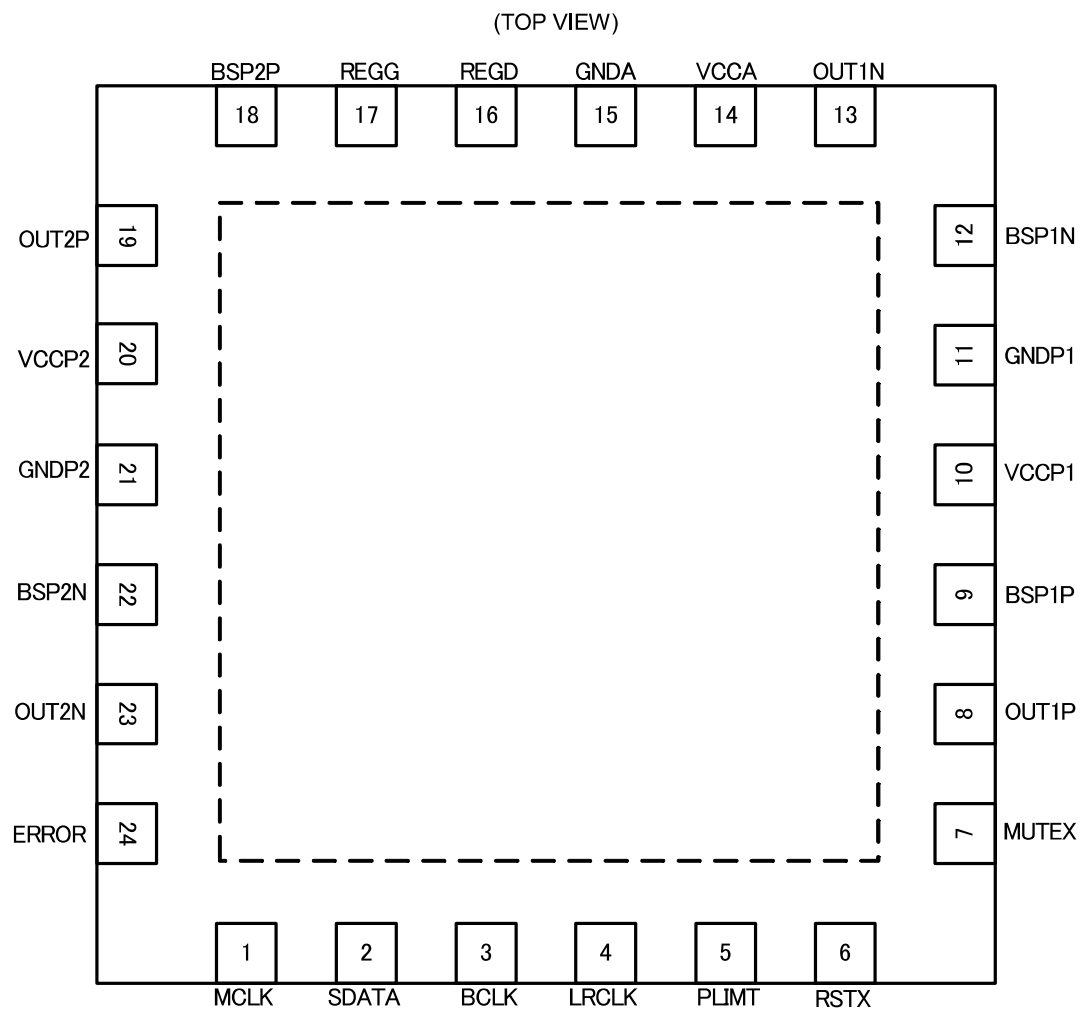
Figure 2. Pin Configuration
