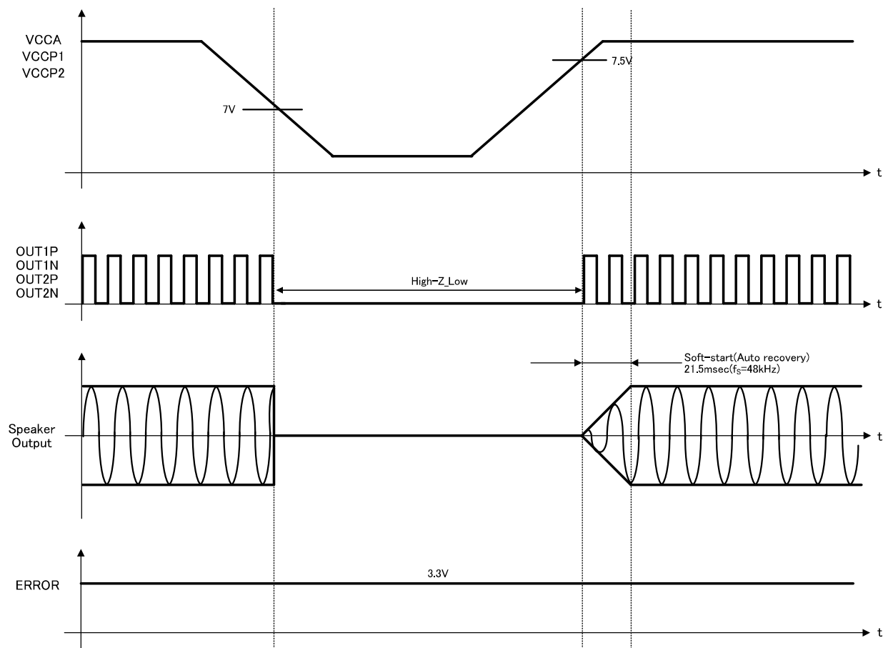
Figure 65. Under Voltage Protection Sequence
