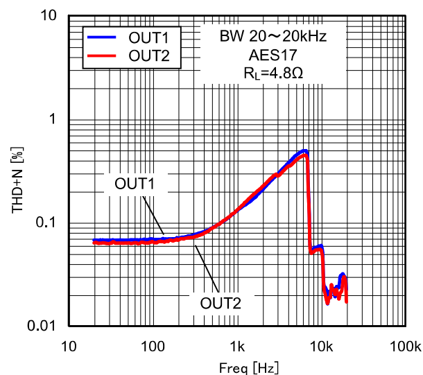
Figure 42. THD+N vs Freq ( 4.8\Omega )
