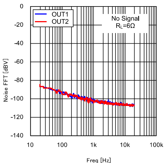
Figure 27. FFT of output noise voltage ( 6\Omega )
