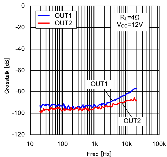
Figure 38. Crosstalk vs Freq ( 4\Omega )
