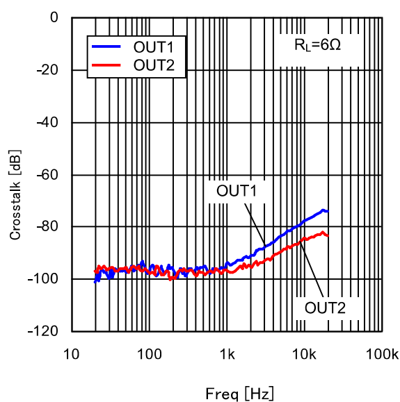
Figure 32. Crosstalk vs Freq ( 6\Omega )
