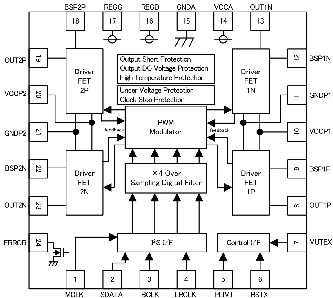
Figure 3. Block Diagram
