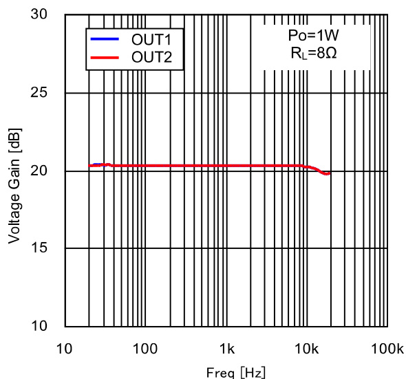
Figure 22. Voltage Gain vs Freq (8Ω)
