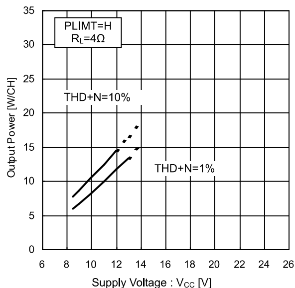
Figure 17. Output Power vs Supply Voltage (4Ω)
