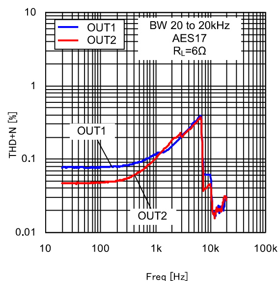
Figure 30. THD+N vs Freq ( 6\Omega )
