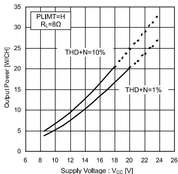
Figure 13. Output Power vs Supply Voltage (8Ω)
