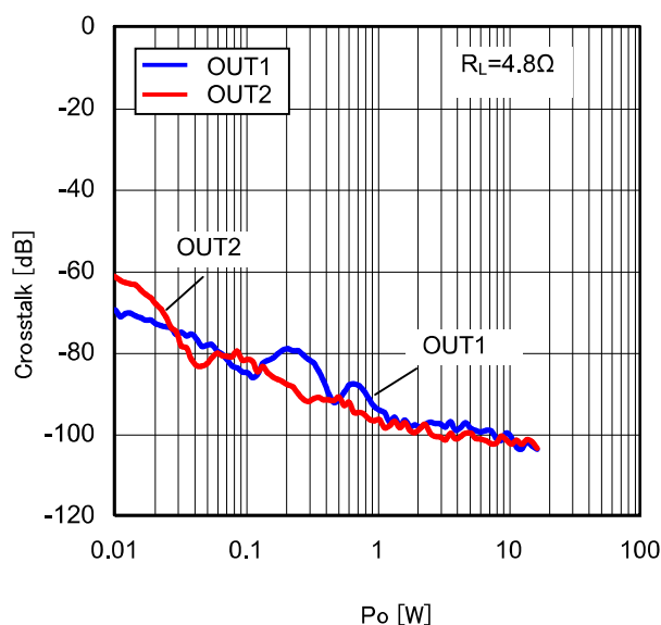
Figure 43. Crosstalk vs P_O ( 4.8\Omega )
