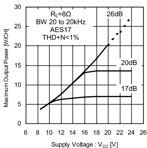
Figure 45. Supply Voltage vs Maximum Output Power (8Ω)
