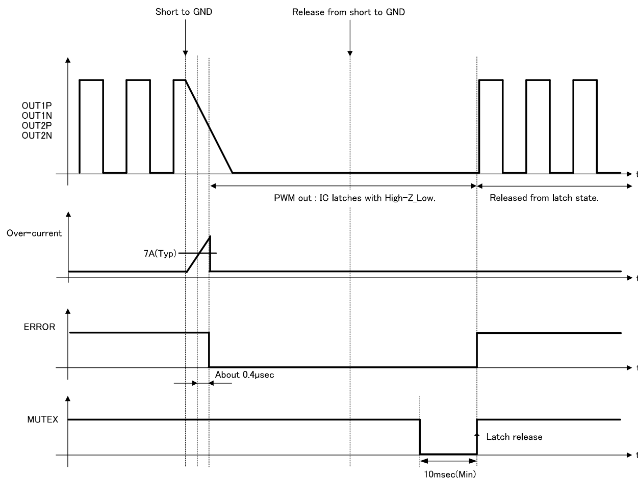
Figure 62. Output Short Protection (Short to GND) Sequence
