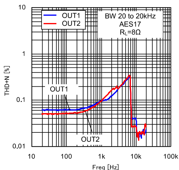
Figure 24. THD+N vs Freq (8Ω)
