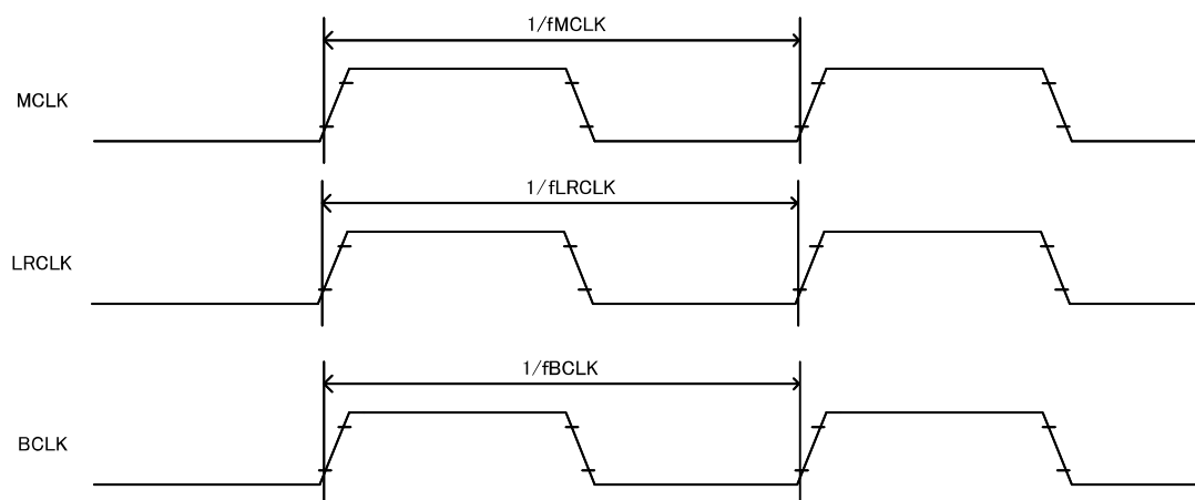
Figure 57. Clock Timing
