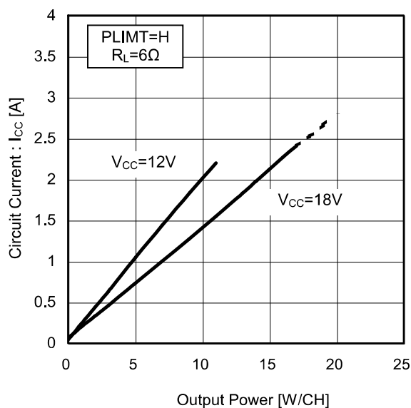
Figure 16. Circuit Current vs Output Power (6Ω)
