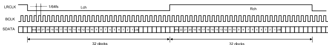
Figure 54. I2S Data Format 64fs, 24bit Data
