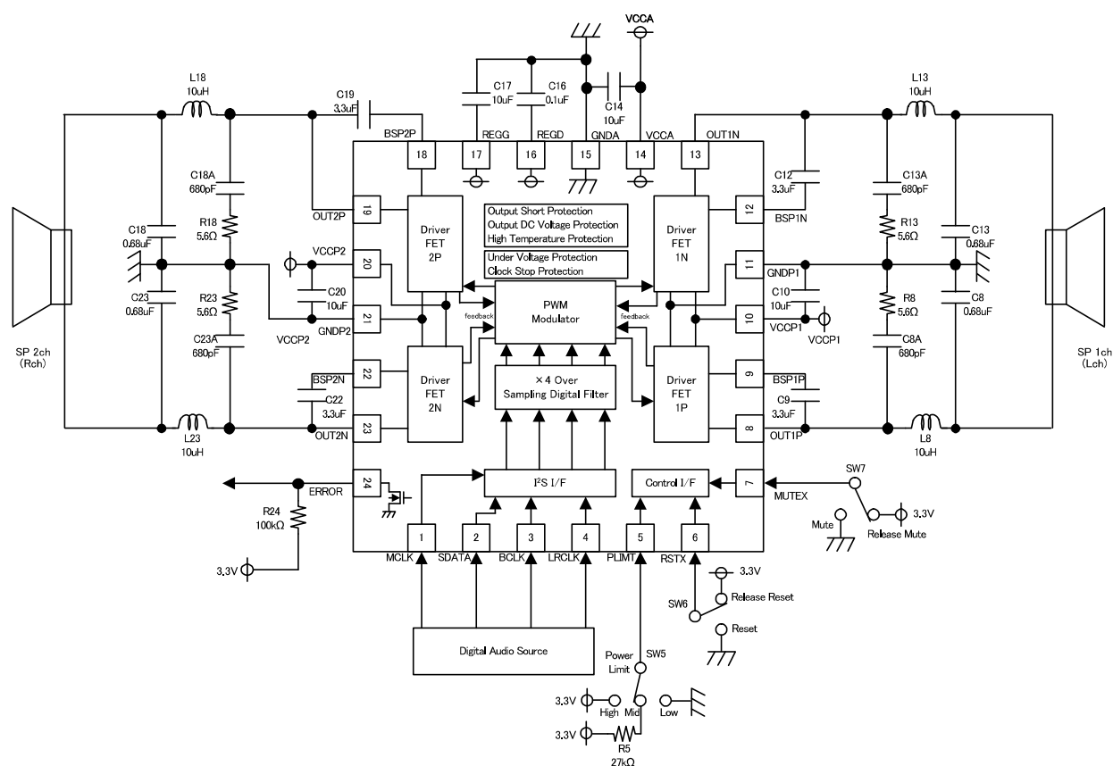
Figure 69. Application Circuit
