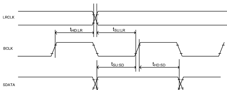
Figure 50 Audio Interface Timing
