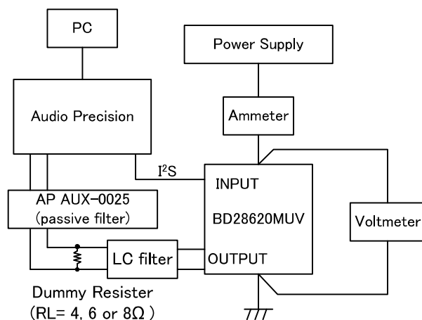
Figure 47. Audio Characteristics Measurement Environment
