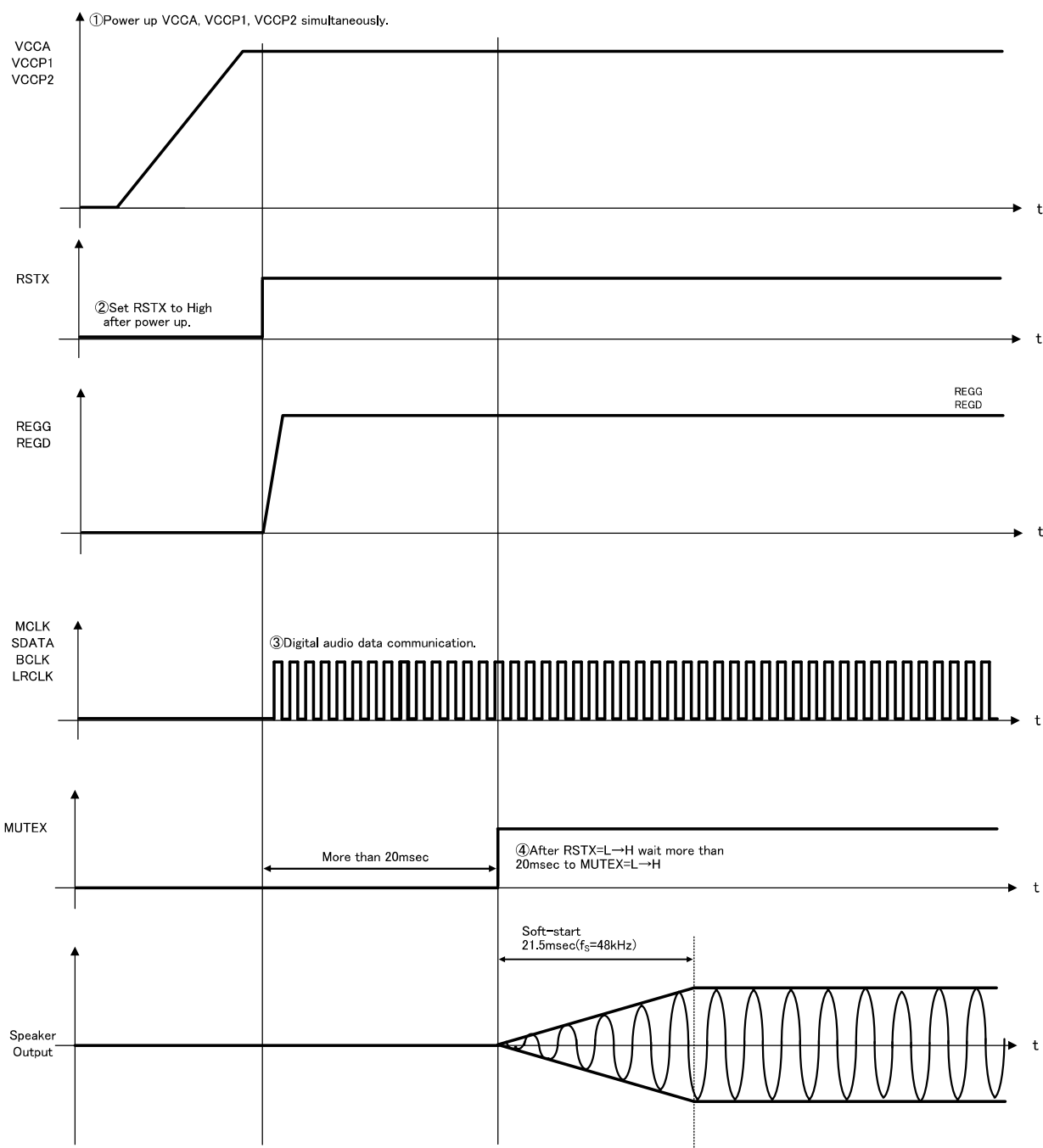
Figure 48. Power Supply Start-up Sequence
