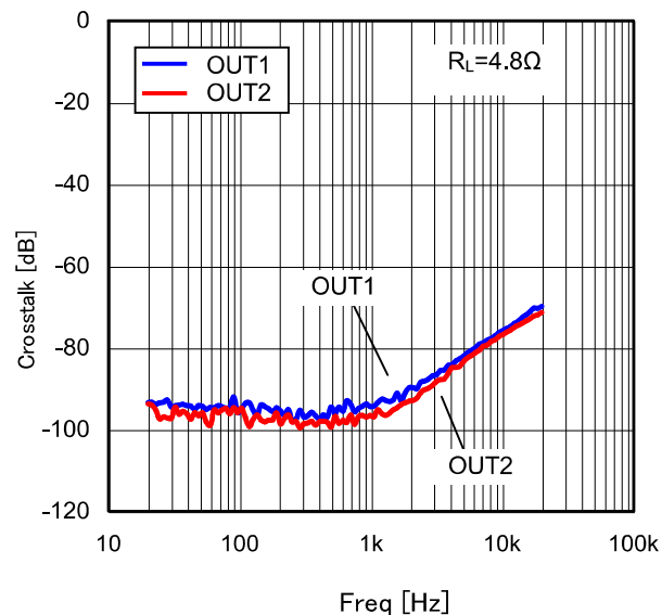
Figure 44. Crosstalk vs Freq ( 4.8\Omega )
