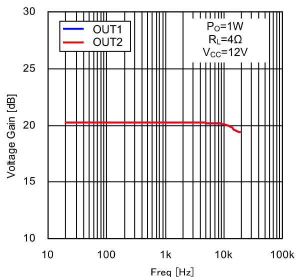
Figure 34. Voltage Gain vs Freq (4Ω)
