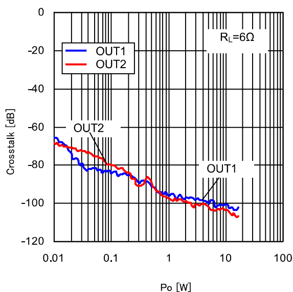
Figure 31. Crosstalk vs P_O ( 6\Omega )
