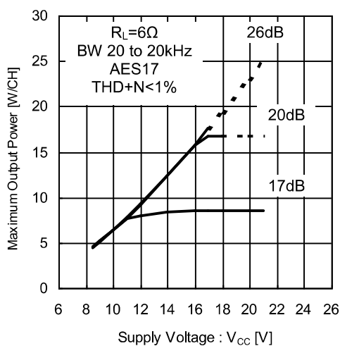
Figure 46. Supply Voltage vs Maximum Output Power (6Ω)
