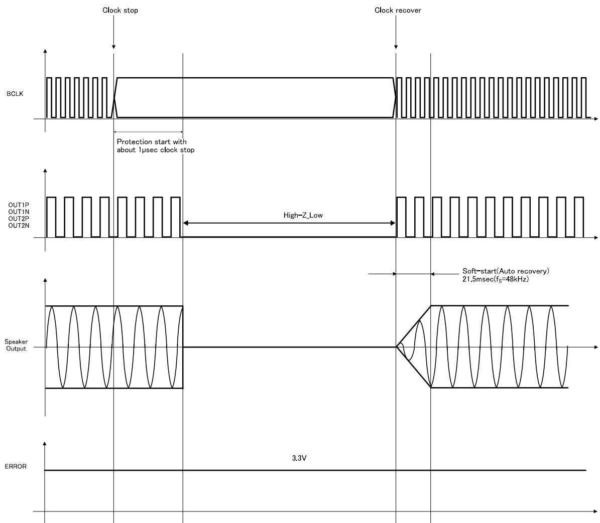
Figure 67. Clock Stop Protection (BCLK) Sequence
