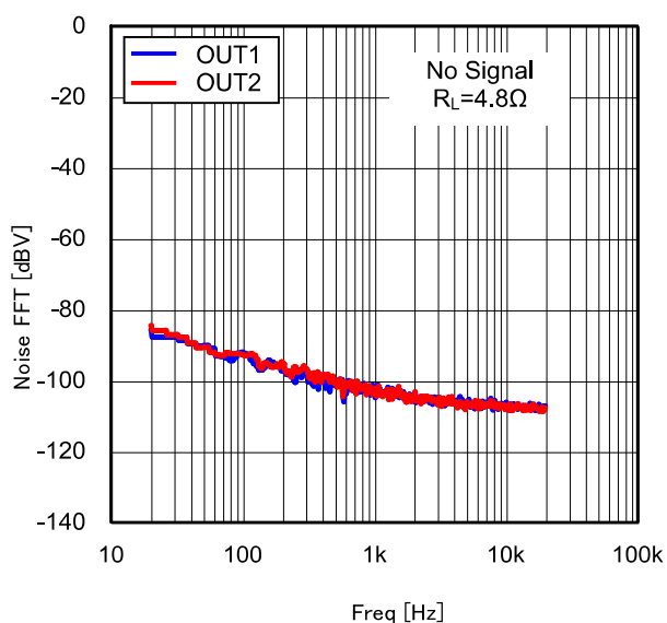
Figure 39. FFT of output noise voltage ( 4.8\Omega )
