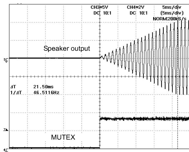
Figure 11. Waveform of Soft Start
