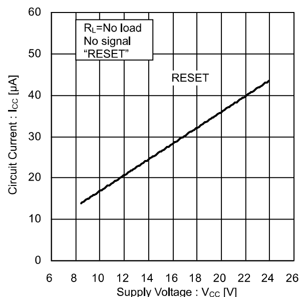
Figure 5. Circuit Current vs Supply Voltage (RESET)
