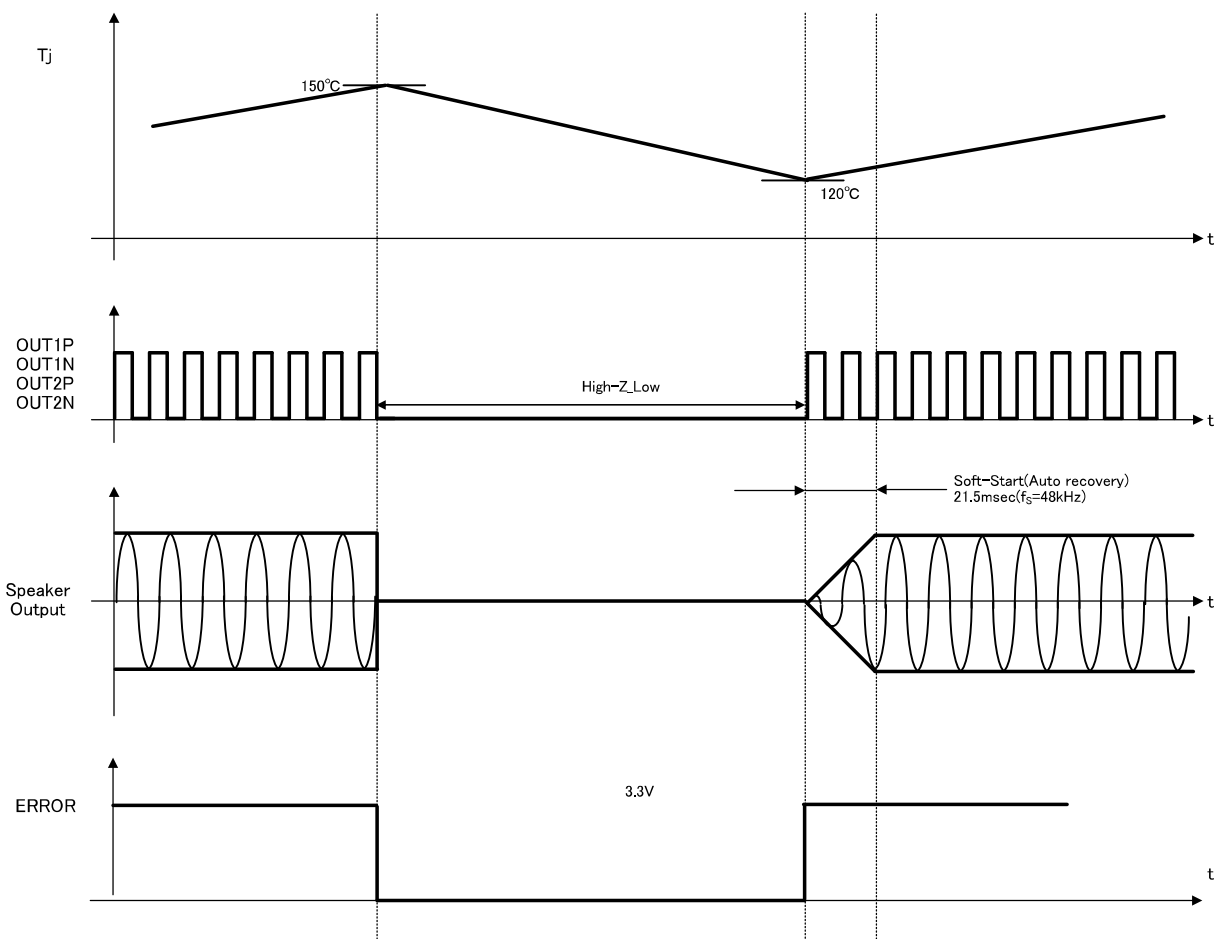
Figure 64. High Temperature Protection Sequence
