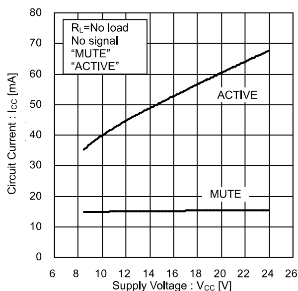
Figure 6. Circuit Current vs Supply Voltage (MUTE, ACTIVE)
