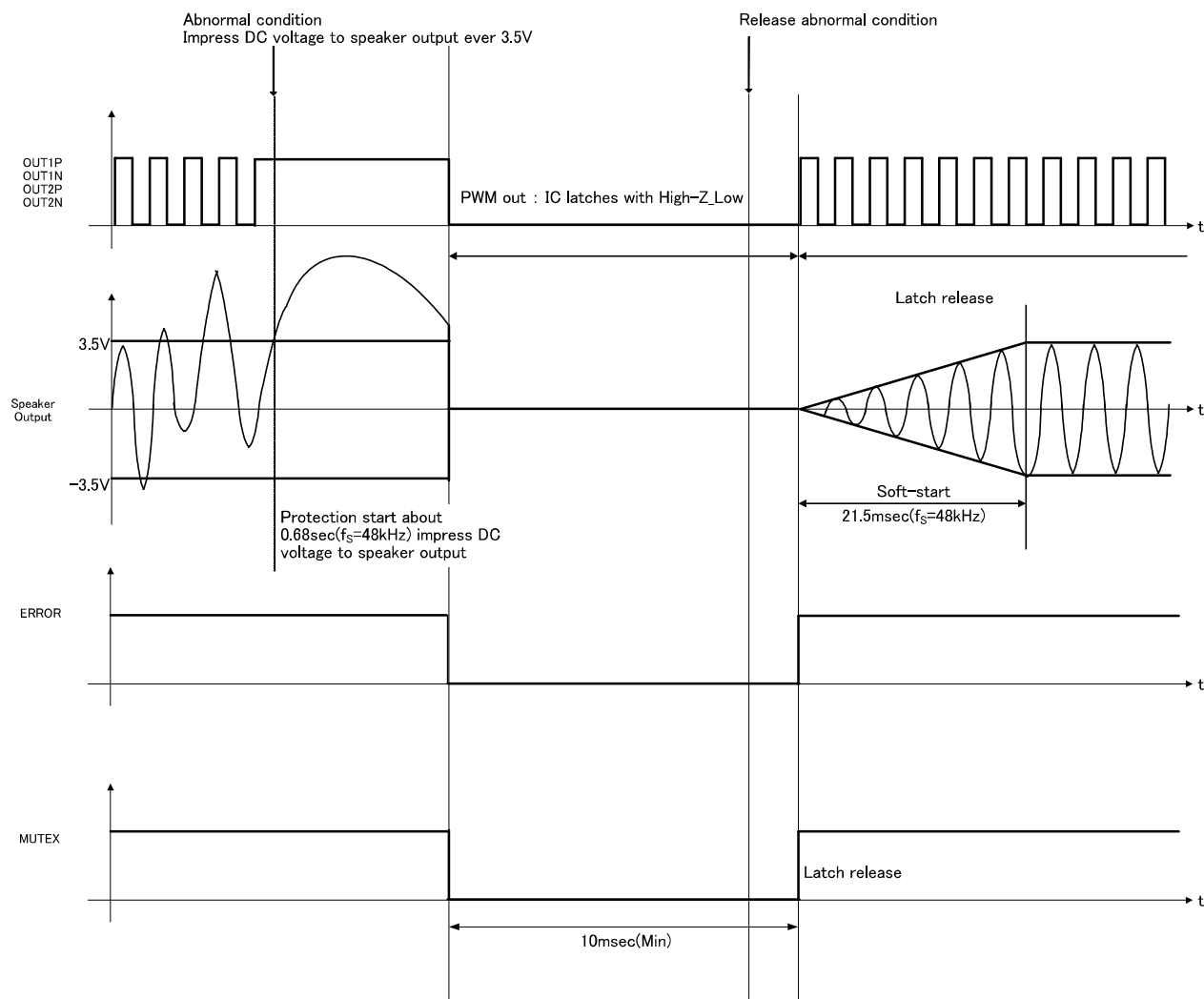
Figure 63. DC Voltage Protection Sequence
