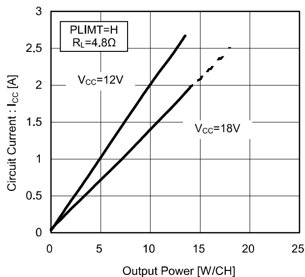
Figure 20. Circuit Current vs Output Power (4.8Ω)
