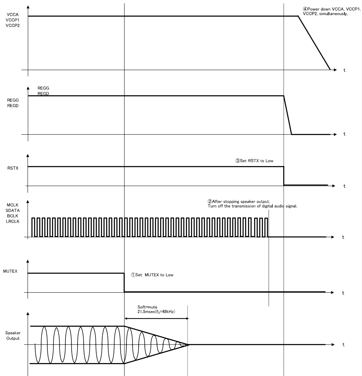
Figure 49. Power Supply Shutdown Sequence
