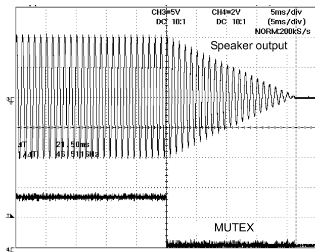
Figure 12. Waveform of Soft Mute
