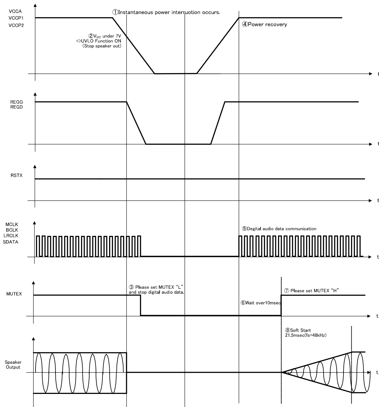
Figure 53. Instantaneous Power Interruption Recovery Sequence
