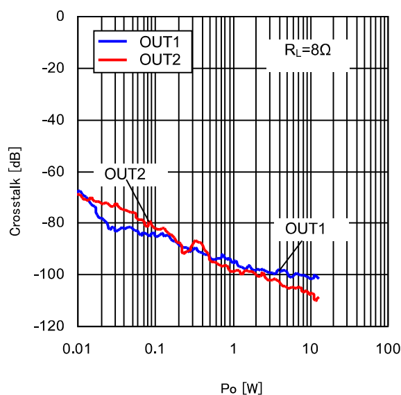
Figure 25. Crosstalk vs P_O ( 8\Omega )
