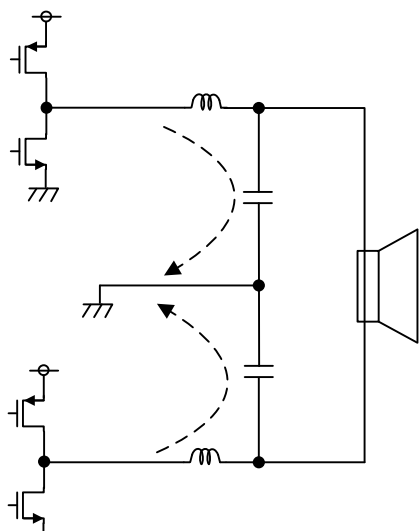
Figure 70. Output LC Filter
