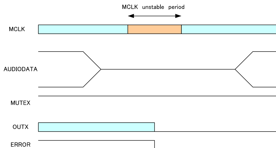
Figure 50. Action at MCLK Unstable 1
