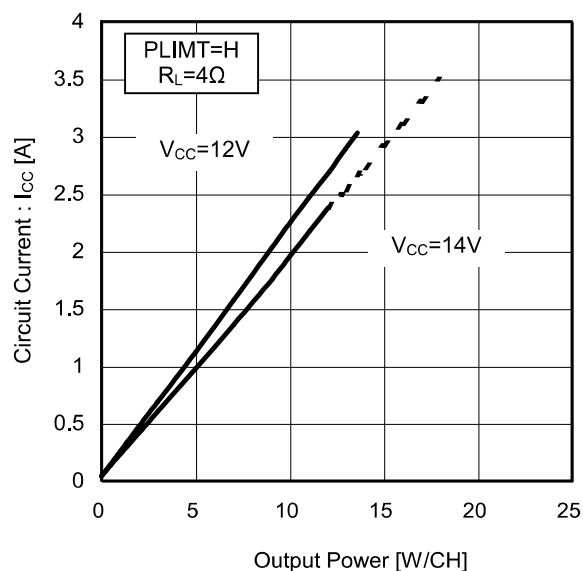
Figure 18. Circuit Current vs Output Power (4Ω)
