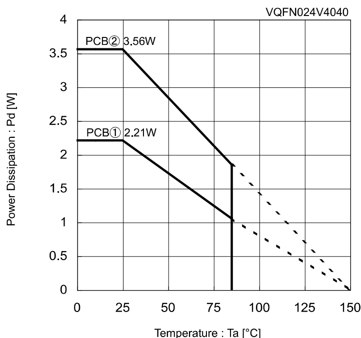
Figure 75. Power Dissipation Curve
