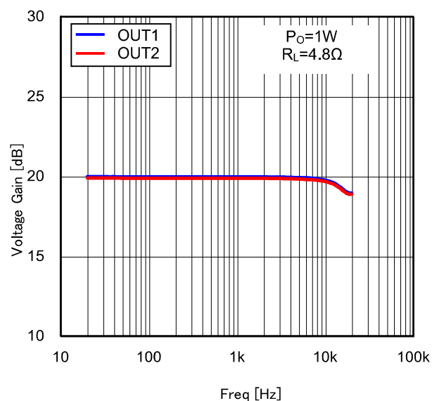
Figure 40. Voltage Gain vs Freq ( 4.8\Omega )
