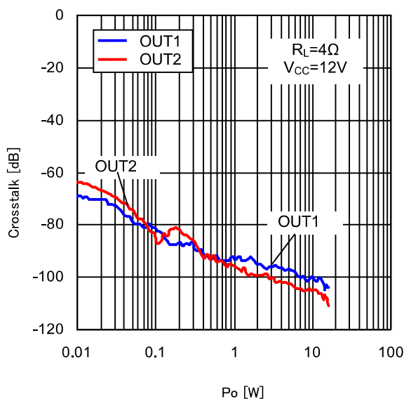
Figure 37. Crosstalk vs P_O ( 4\Omega )
