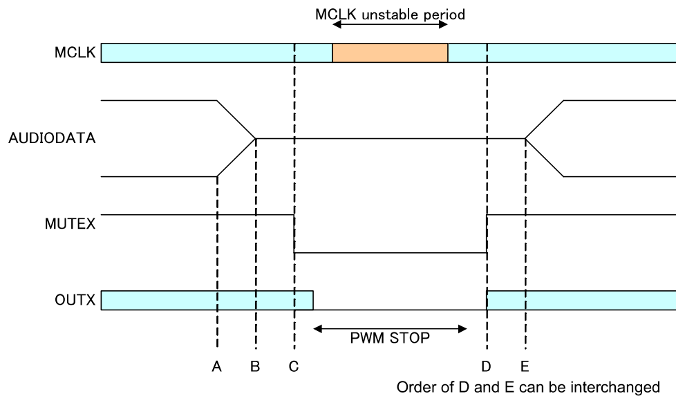
Figure 51. Action at MCLK Unstable 2
