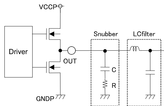
Figure74. Snubber Schematic
