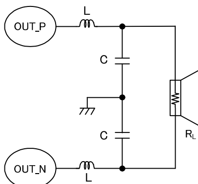
Figure 72. Output LC Filter
