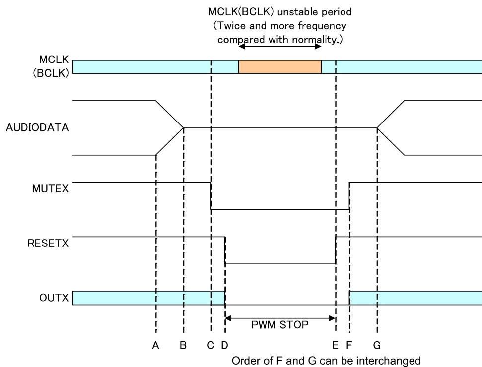
Figure 52. Action at MCLK Unstable 3
