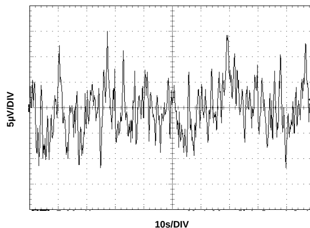
FIGURE 14. V_{OUT} NOISE
