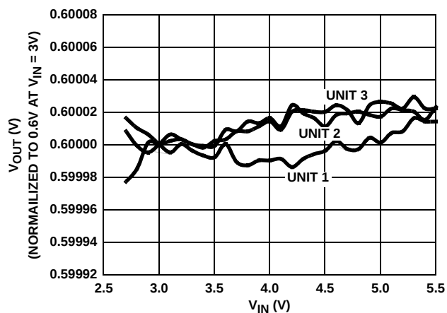
FIGURE 4. LINE REGULATION
