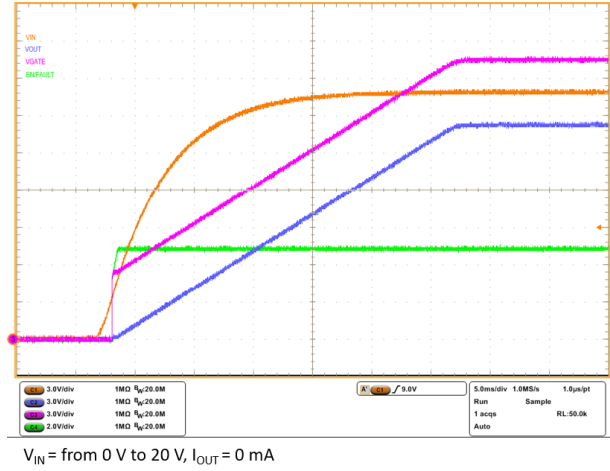
Figure 26. Startup into voltage clamp
