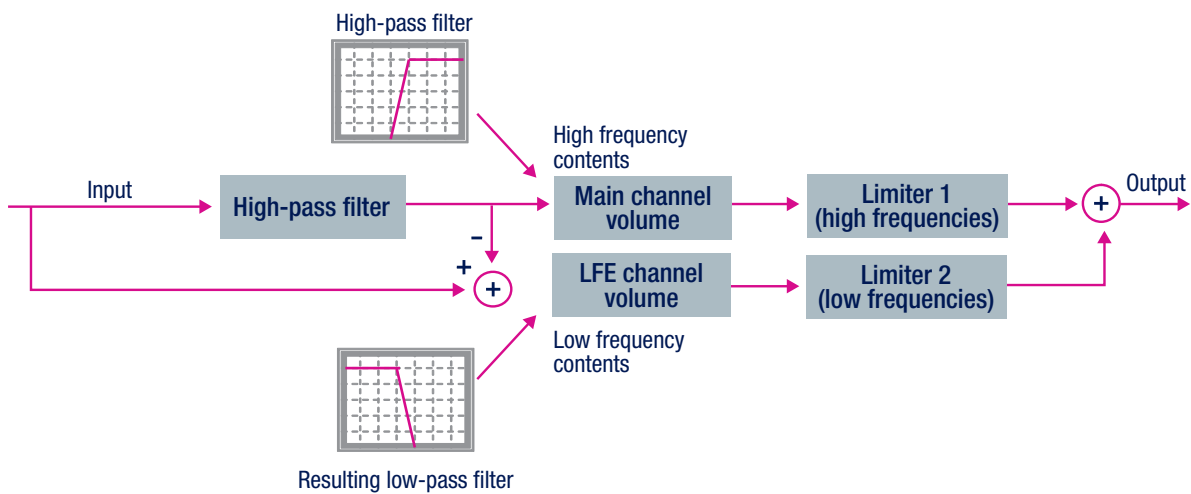
Figure 2: Dual-band DRC (depicted for a single channel only)
