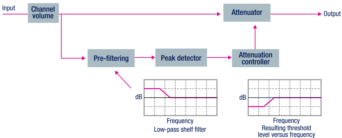
Figure 3: EqDRC block diagram
