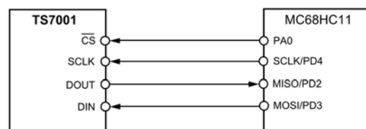
Figure 18: Interfacing the TS7001 to 68HC11-type Microcontrollers.
