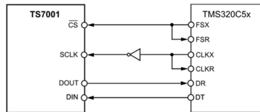
Figure 15: Interfacing the TS7001 to TMS320C5x-type DSPs.
