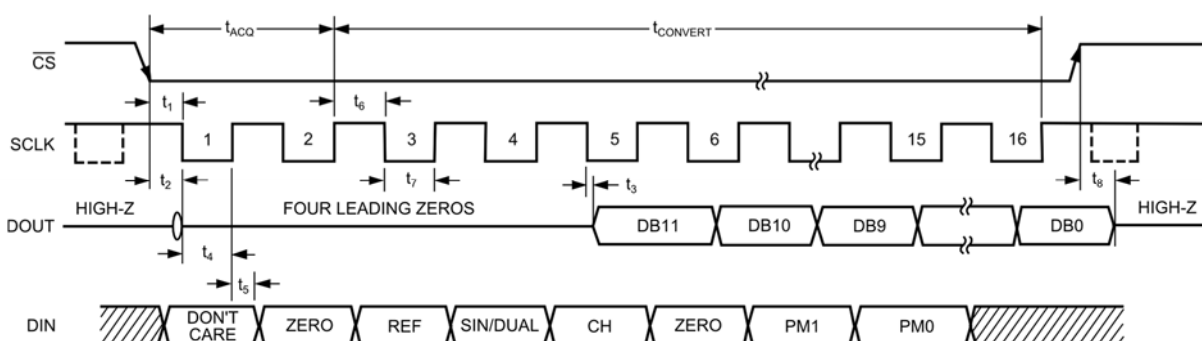
Figure 14: TS7001's Detailed Serial Interface Timing Diagram.
