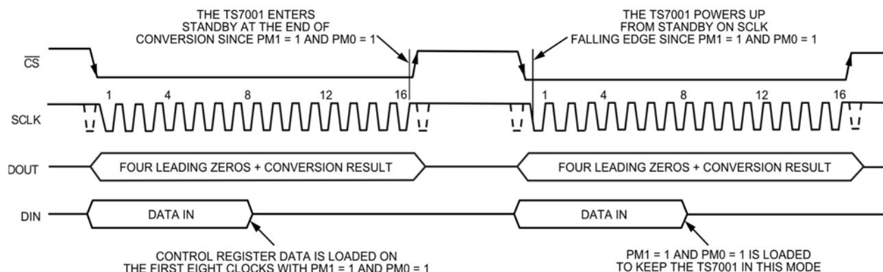
Figure 13: TS7001's Power Management Mode 4 Operation Diagram.
