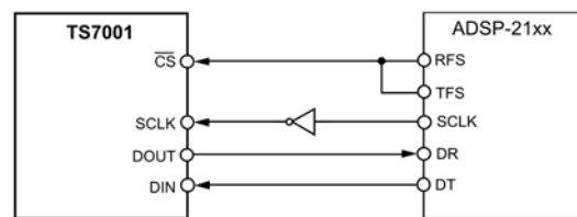
Figure 16: Interfacing the TS7001 to ADSP-21xx-type DSPs.
