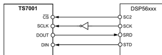
Figure 17: Interfacing the TS7001 to DSP56xxx-type DSPs.
