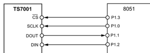
Figure 19: Interfacing the TS7001 to Legacy 8051-type Microcontrollers.
