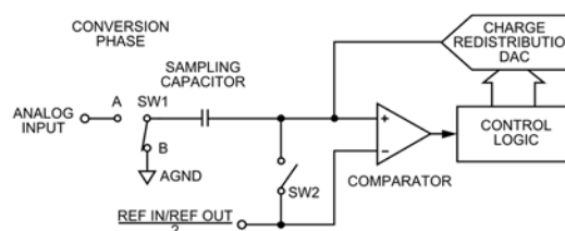
Figure 2: TS7001's Conversion Phase Equivalent Circuit
