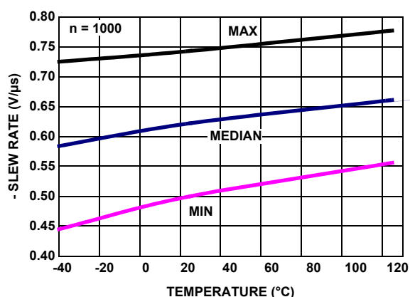
FIGURE 48. - SLEW RATE vs TEMPERATURE, INPUT = \pm 0.15V AT GAIN = +10
