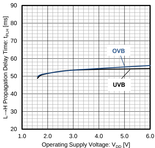
Figure 11. L→H Propagation Delay Time vs Operating Supply Voltage ( T_a = 25\text{ }^{\circ}\text{C} , C_{CT} = 10\text{ nF} )
