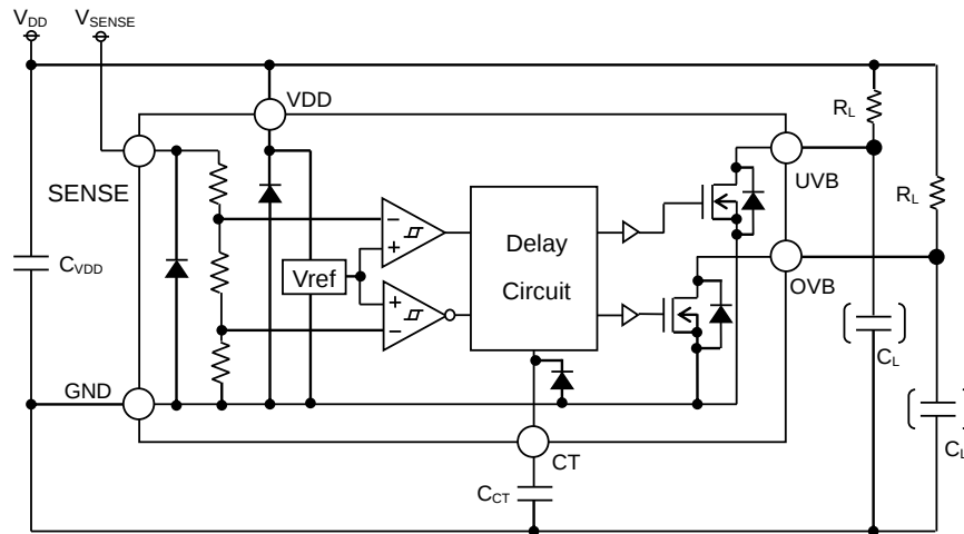
Figure 17. Set-up diagram
