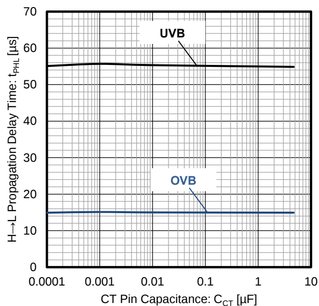
Figure 16. H→L Propagation Delay Time vs CT Pin Capacitance ( V_{DD} = 3 V , T_a = 25^\circ C )
