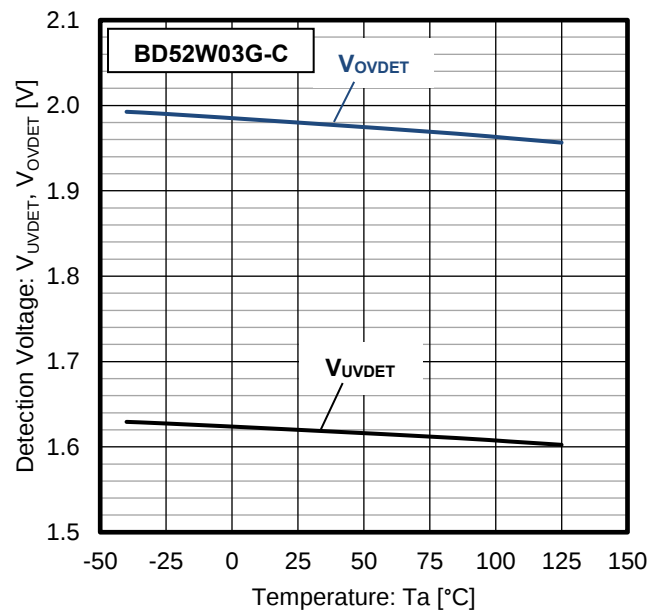
Figure 4. Detection Voltage vs Temperature ( V_{DD} = 3\text{ V} )
