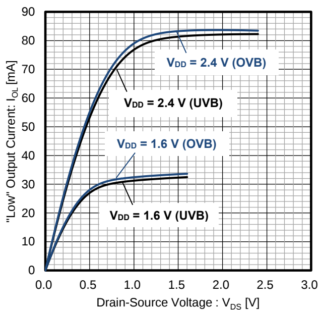
Figure 9. "Low" Output Current vs Drain-Source Voltage ( T_a = 25\text{ }^{\circ}\text{C} )
