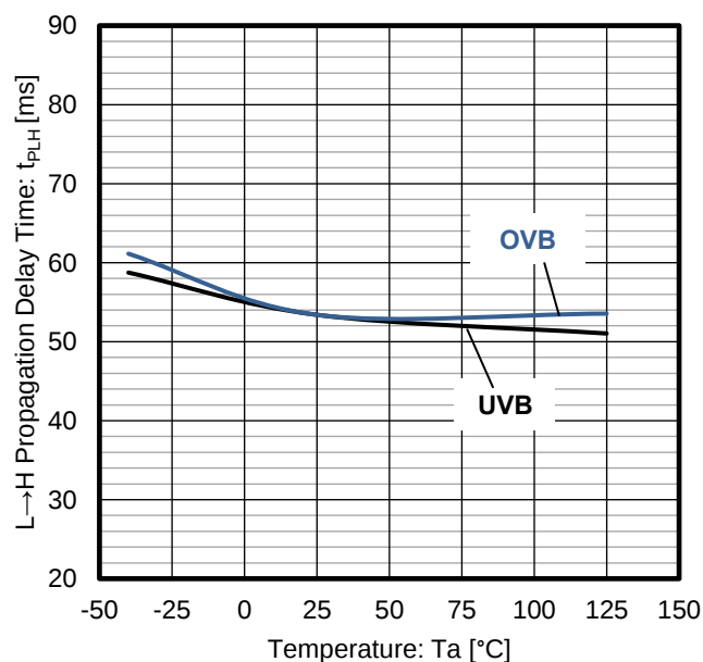
Figure 12. L→H Propagation Delay Time vs Temperature ( V_{DD} = 3\text{ V} , C_{CT} = 10\text{ nF} )
