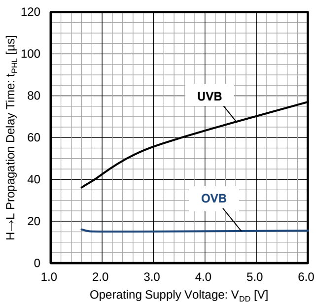
Figure 13. H→L Propagation Delay Time vs Operating Supply Voltage ( T_a = 25^\circ C )
