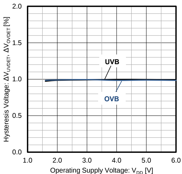
Figure 5. Hysteresis Voltage vs Operating Supply Voltage ( T_a = 25^\circ\text{C} )
