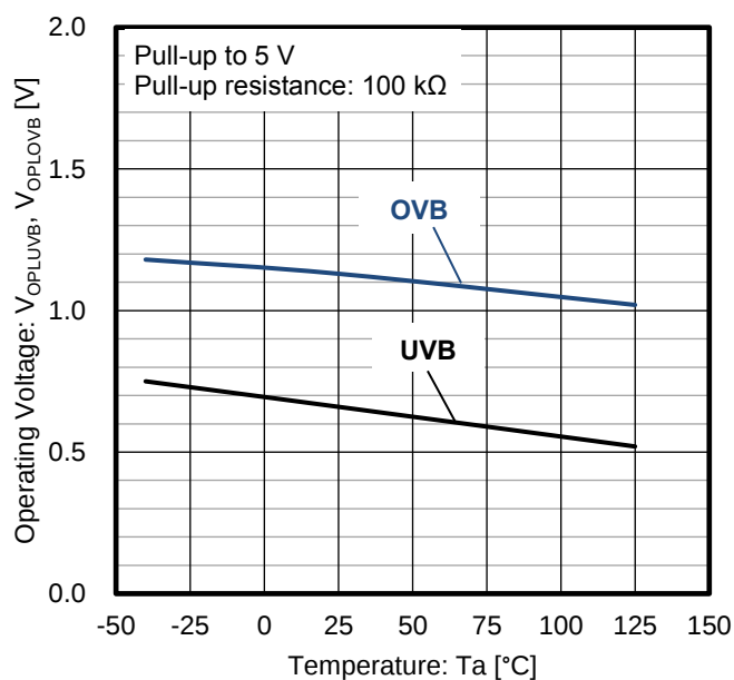
Figure 8. Operating Voltage vs Temperature
