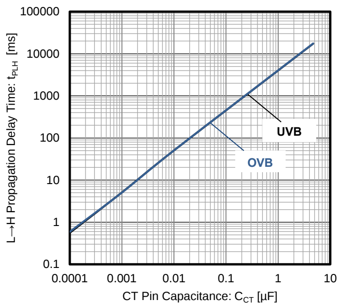
Figure 15. L→H Propagation Delay Time vs CT Pin Capacitance ( V_{DD} = 3 V , T_a = 25^\circ C )
