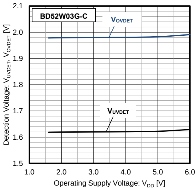
Figure 3. Detection Voltage vs Operating Supply Voltage ( T_a = 25\text{ °C} )
