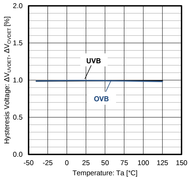
Figure 6. Hysteresis Voltage vs Temperature ( V_{DD} = 3\text{ V} )
