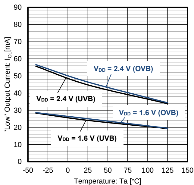
Figure 10. "Low" Output Current vs Temperature ( V_{DS} = 0.4\text{ V} )
