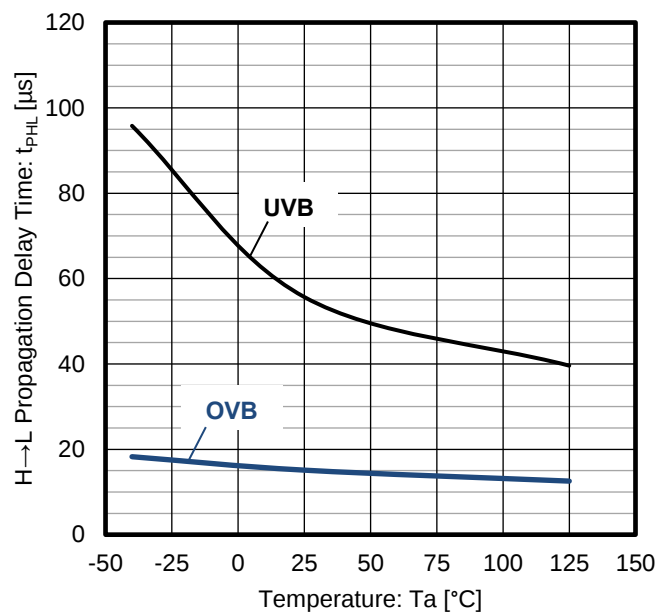
Figure 14. H→L Propagation Delay Time vs Temperature ( V_{DD} = 3 V )
