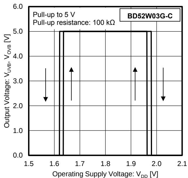
Figure 7. Output Voltage vs Operating Supply Voltage ( T_a = 25^\circ\text{C} , V_{DD} = \text{SENSE} , \text{UVB} = \text{OVB} )
