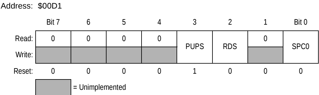
Figure 13-5. SPI Control Register 2 (SP0CR2)
