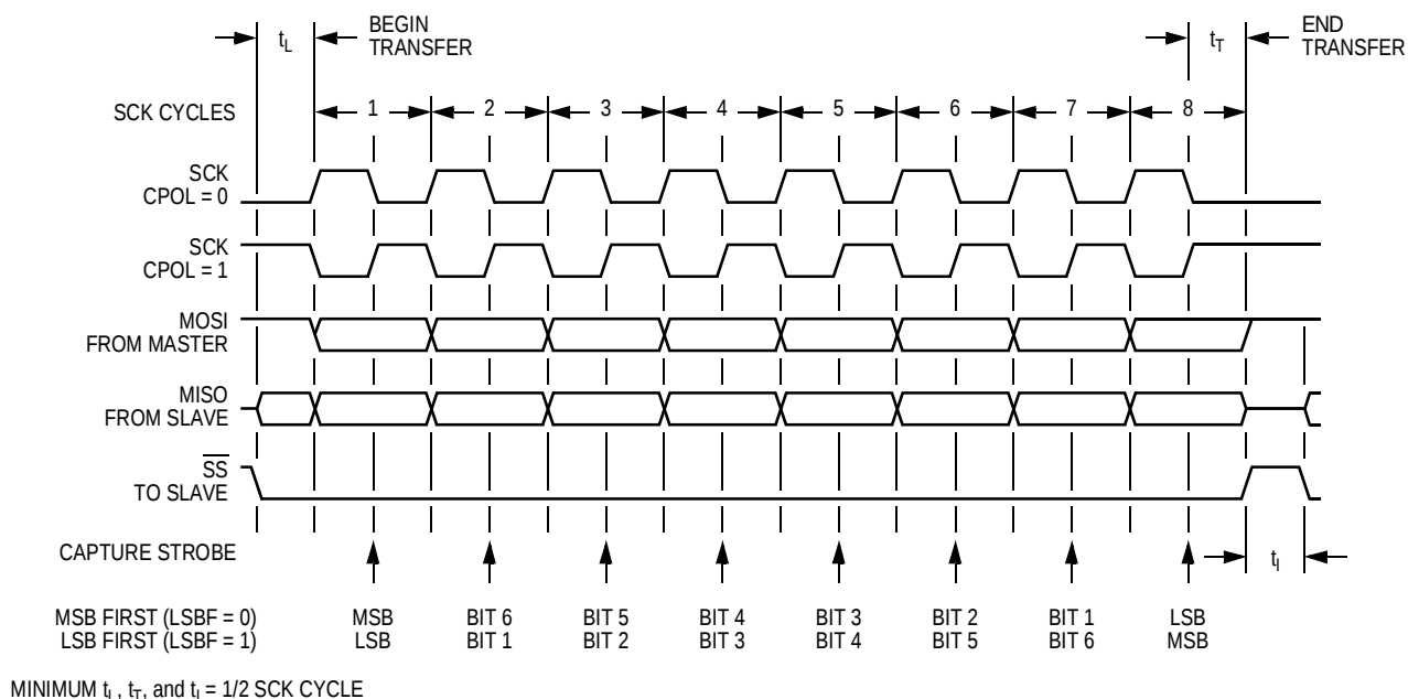
Figure 15-6. Transmission Format 1 ( \text{CPHA} = 1 )
