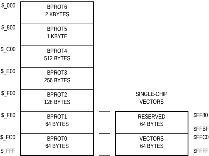
Figure 7-1. EEPROM Block Protect Mapping
