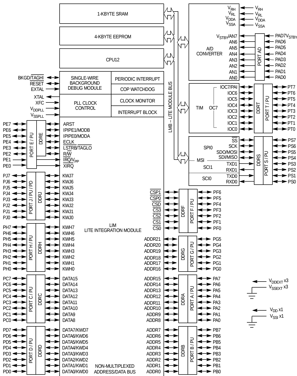
Figure 1-1. Block Diagram
