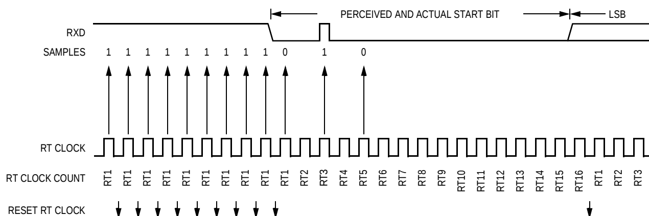
Figure 14-10. Start Bit Search Example 4
