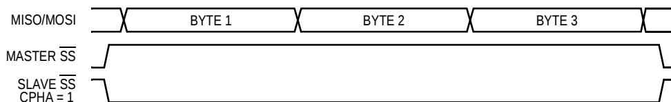
Figure 15-7. Slave \overline{\text{SS}} When \text{CPHA} = 1
