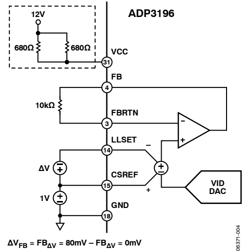
Figure 4. Positioning Voltage
