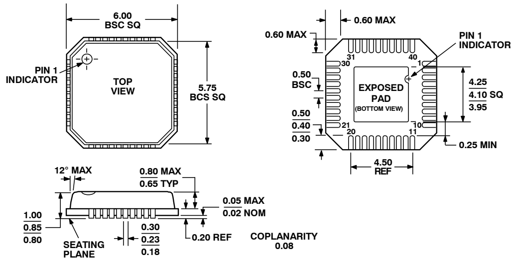
COMPLIANT TO JEDEC STANDARDS MO-220-VJJD-2 Figure 12. 40-Lead Lead Frame Chip Scale Package [LFCSP_VQ] 6 mm × 6 mm Body, Very Thin Quad (CP-40) Dimensions shown in millimeters
