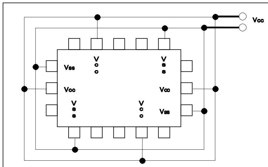
Figure 7-1 Pin Assignment
