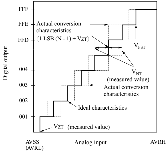
Integral linearity error
