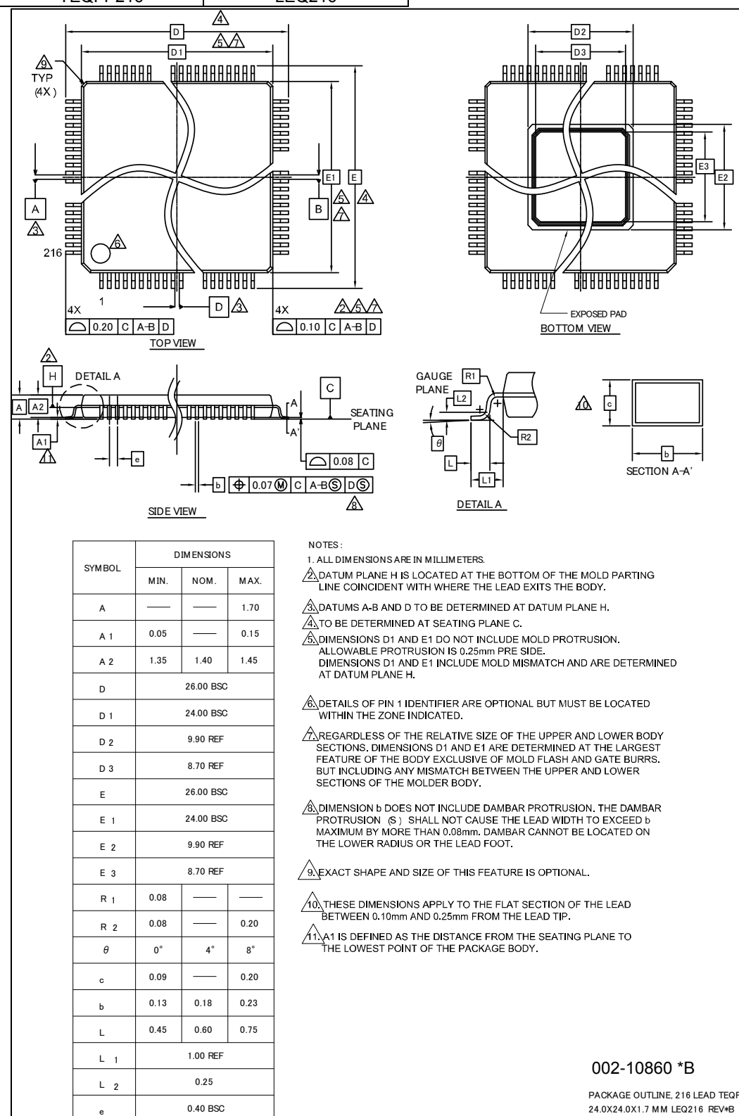
Figure 4-19 LEQ216
