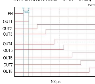
DAISY-CHAINING TWO DEVICES WITH EN RISING (CDLY = CPGT = OPEN)
