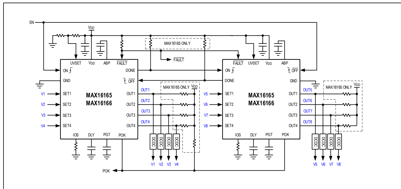
Figure 13. Sequence and Monitor Eight Power Supplies and Monitor V_{PP} .
