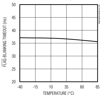
FLAG-BLANKING TIMEOUT vs. TEMPERATURE
