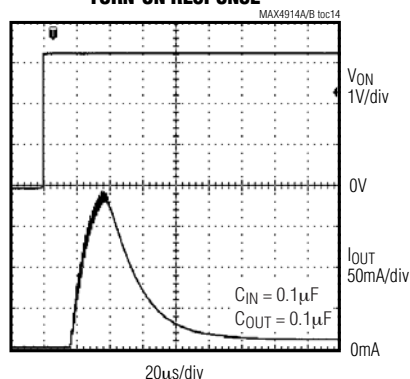
TURN-ON RESPONSE
