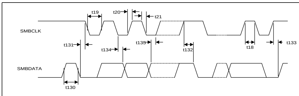
Figure 8-21. SMBus Timeout
