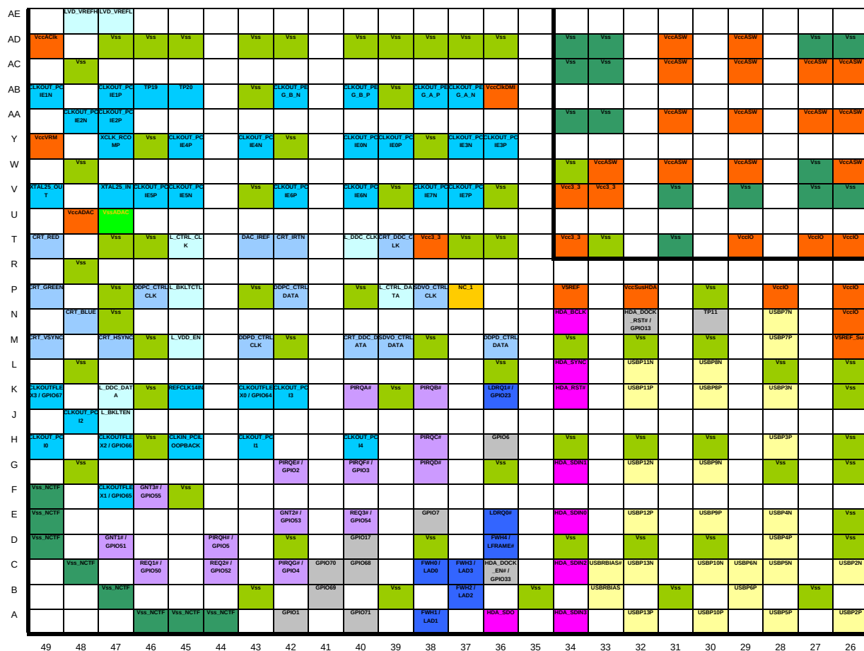
Figure 6-6. Mobile PCH Ballout (Top View - Lower Left)
