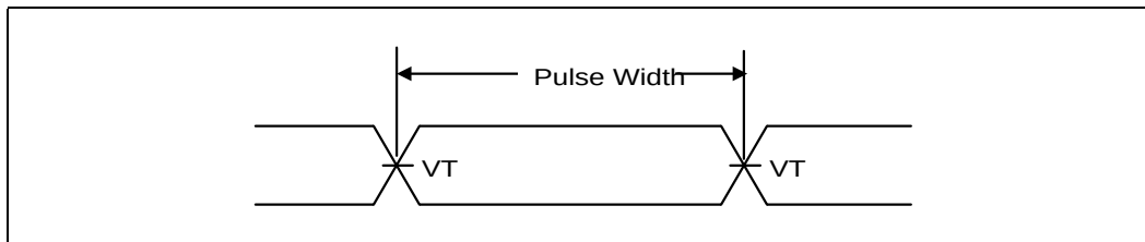
Figure 8-15. Pulse Width
