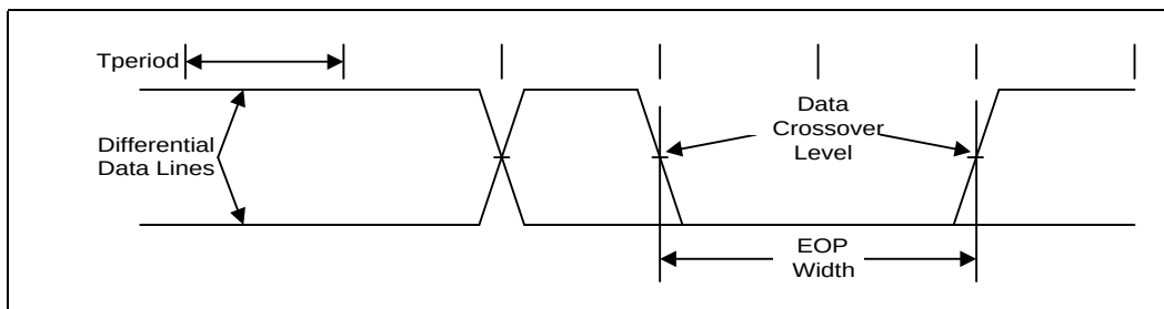
Figure 8-20. SMBus Transaction
