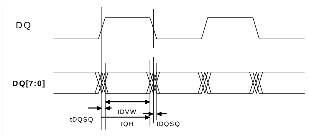
Figure 8-25. Dual Channel Interface Timings
