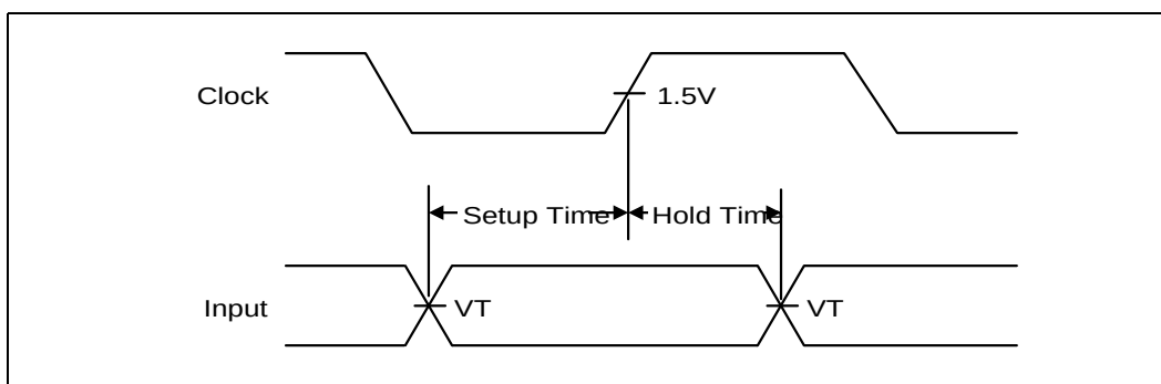
Figure 8-14. Float Delay
