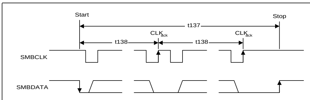
Figure 8-21. SMBus Timeout
