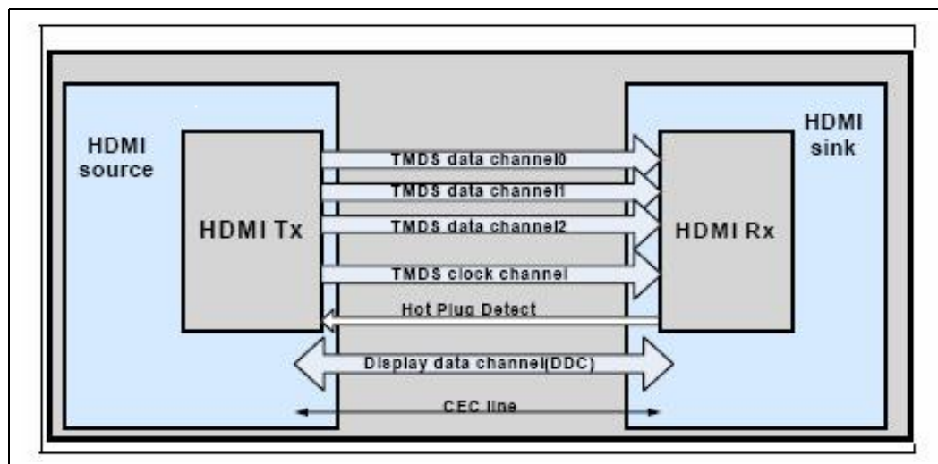
Figure 5-17. HDMI Overview
