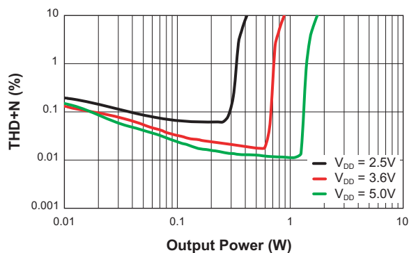
THD+N vs. Output Power (f = 1kHz; R_L = 8\Omega ; Gain = 24dB)
