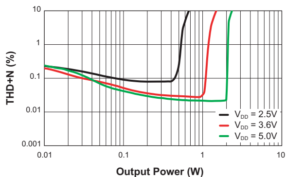
THD+N vs. Output Power (f = 1kHz; R_L = 4\Omega ; Gain = 24dB)
