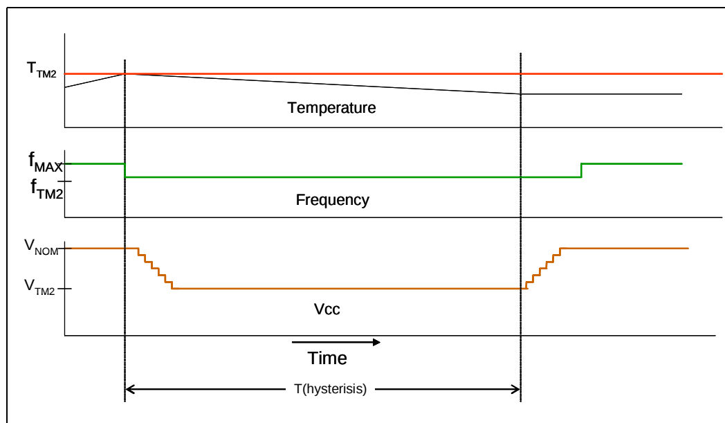
Figure 6-5. Demand Based Switching Frequency and Voltage Ordering
