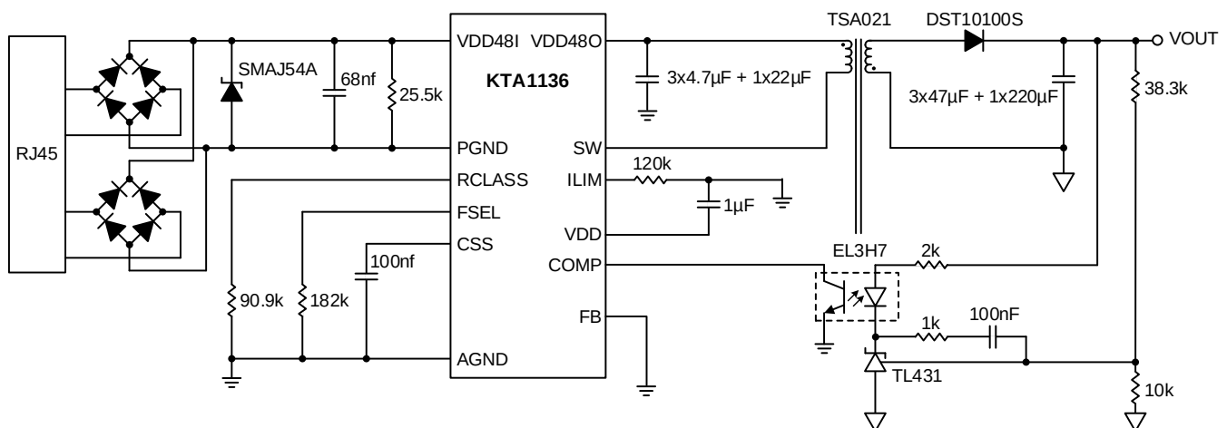
Figure 4. Flyback Application with Secondary Side Regulation
