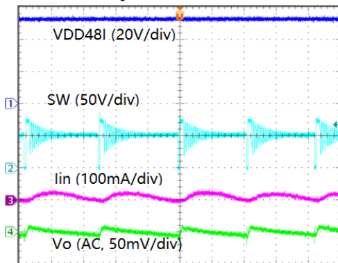
Steady State at 0A Load
