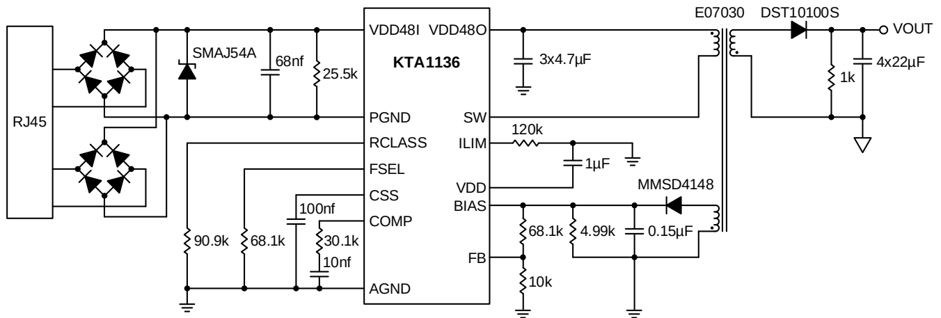
Figure 3. Flyback Application with Primary Side Feedback
