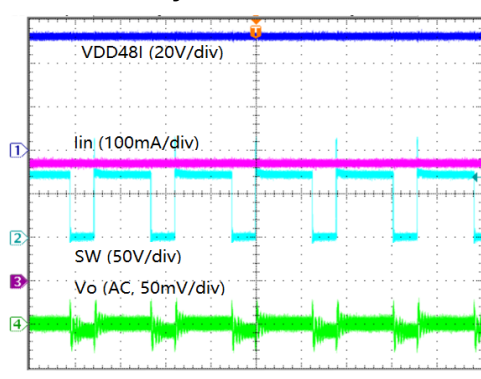
Steady State at 1A Load
