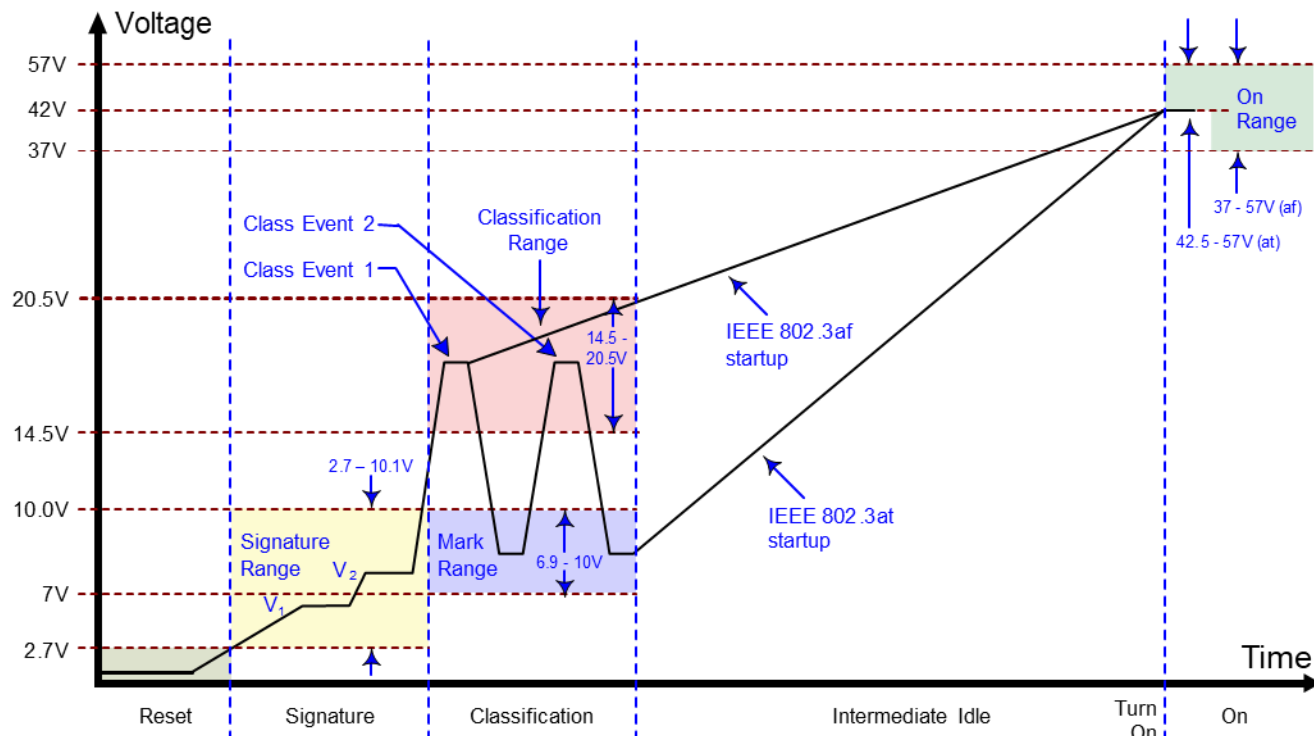
Figure 2. 802.3at Typical Power-On Waveform
