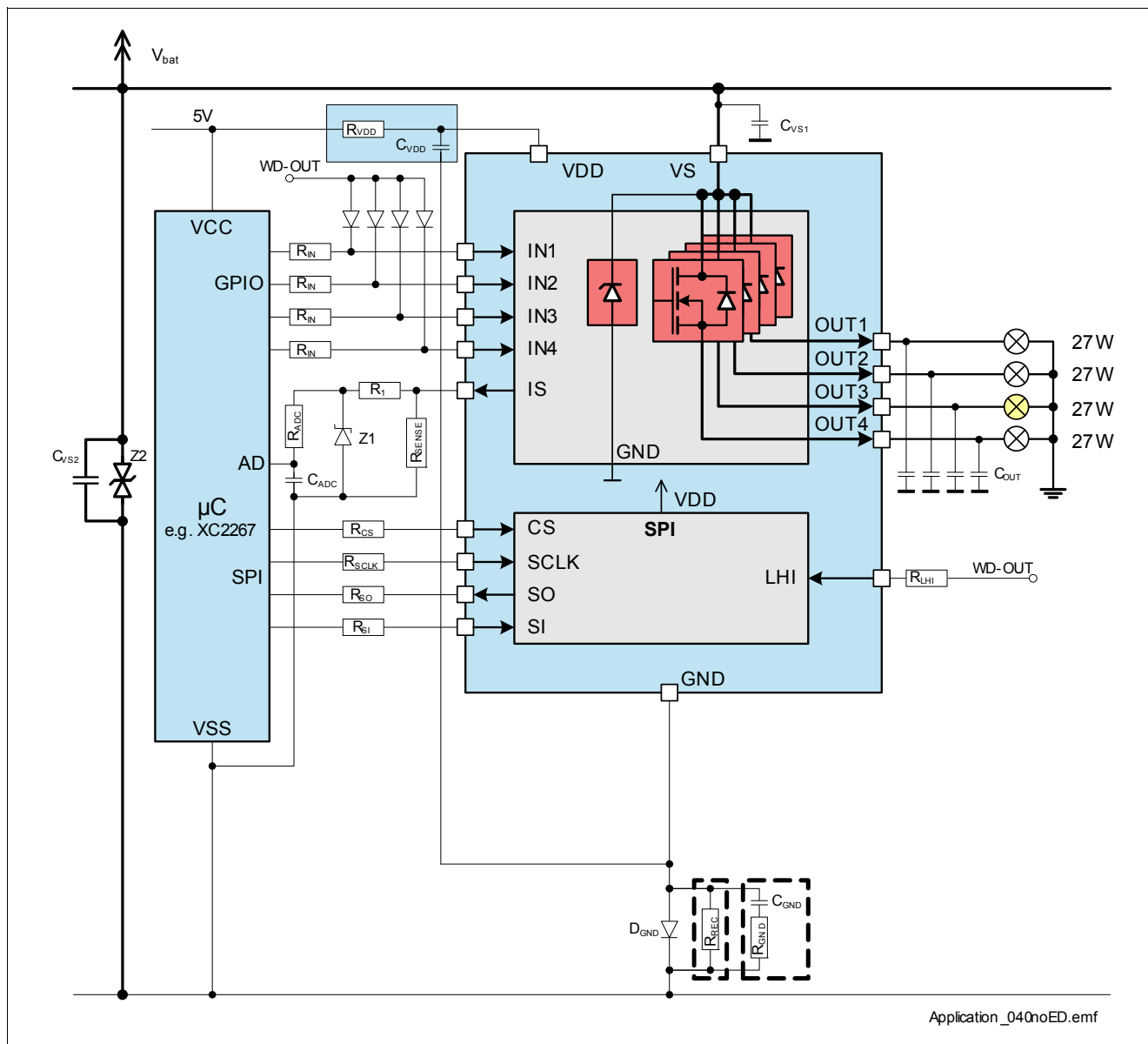
Figure 35 Application Circuit Example
