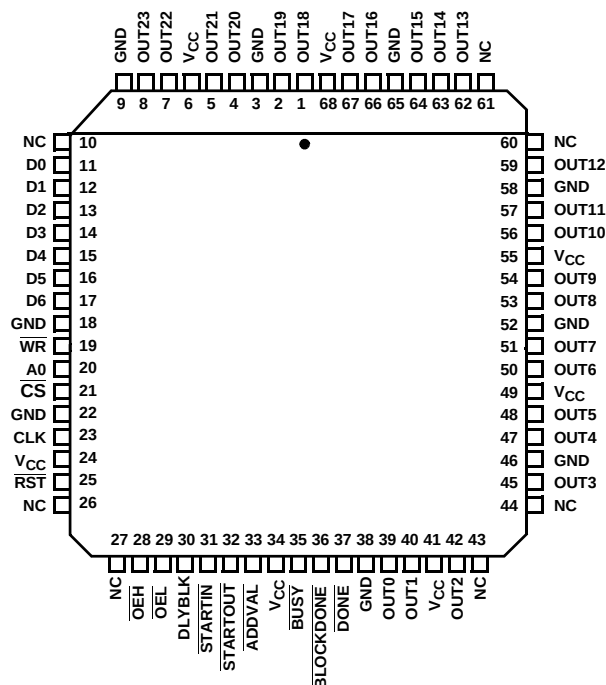
ADDRESS SEQUENCER HSP45240 68 PIN PLASTIC LEADED CHIP CARRIER (PLCC)
