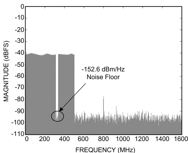
Wideband Performance
