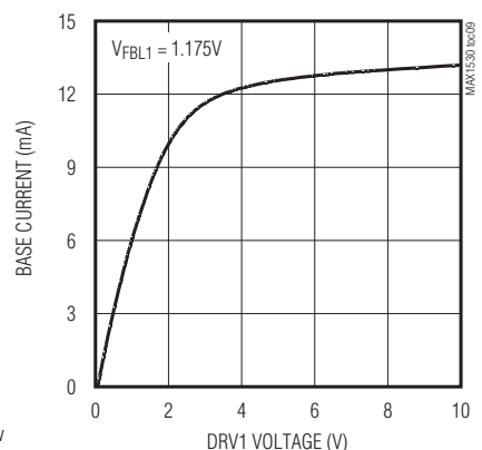
LR1 BASE CURRENT vs. DRV1 VOLTAGE
