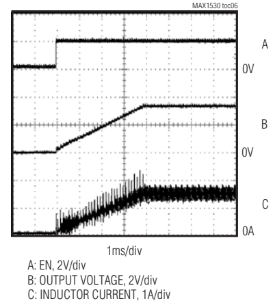
STEP-DOWN REGULATOR SOFT-START
