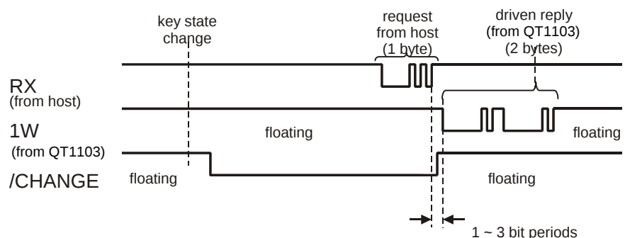
Figure 2.9 2W Operation
