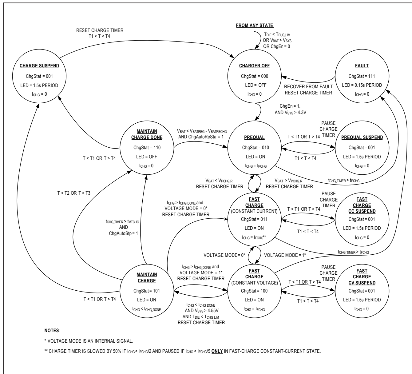
Figure 5. Battery Charger State Diagram
