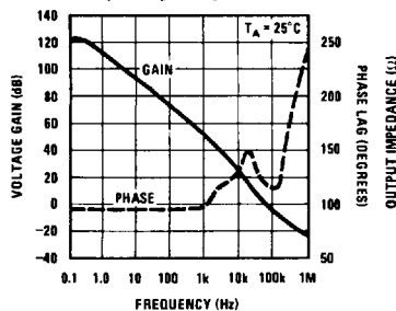
Frequency Response
