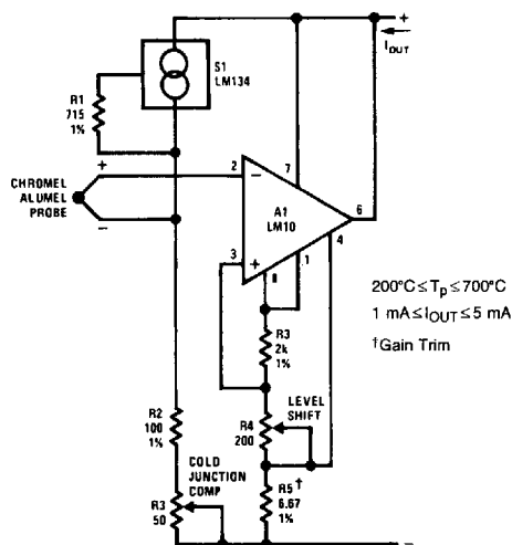
Thermocouple Transmitter
