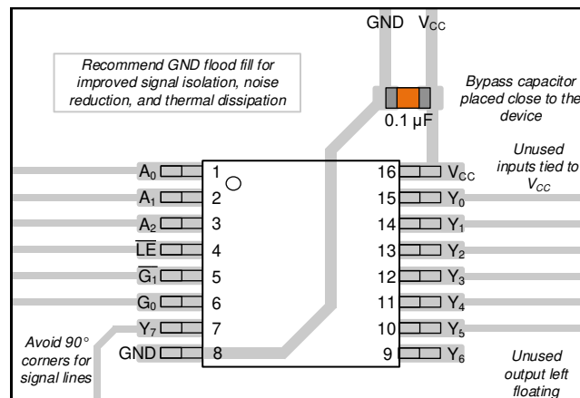
Figure 11-1. Example layout for the SN74HCS137 in the PW package.
