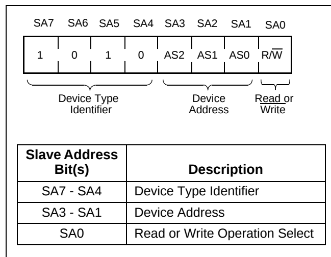
Figure 15. Slave Address (SA) Format
