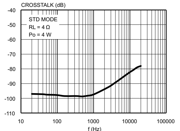
Figure 20. Crosstalk vs. frequency (STD mode)
