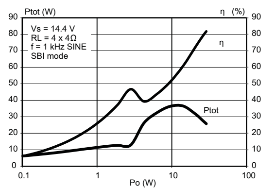
Figure 24. Total power dissipation & efficiency vs. P_o (4 Ω, SBI, Sine)
