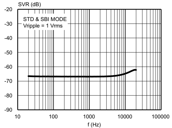
Figure 22. Supply voltage rejection vs. frequency
