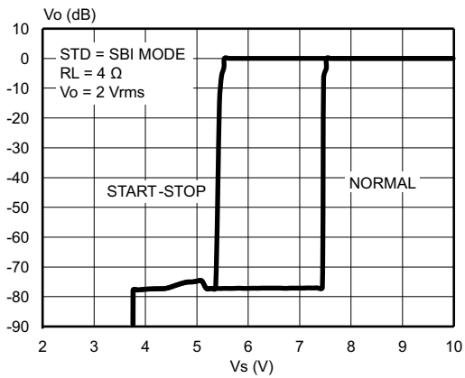
Figure 19. Output attenuation vs. V_s
