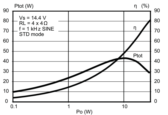
Figure 23. Total power dissipation & efficiency vs. P_o (4 Ω, STD, Sine)
