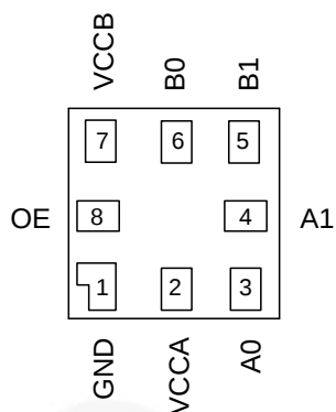
Figure 2. MicroPak™ (Top-Through View)
