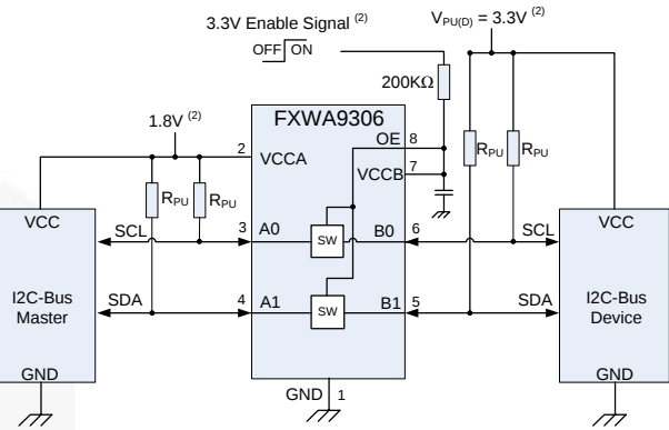
Figure 6. Application (Switch Enable Control)
