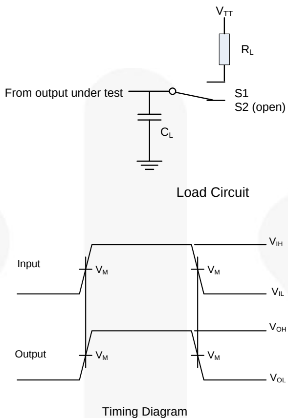
Figure 4. Load Circuit
