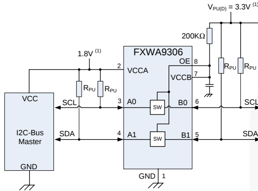
Figure 5. Application (Switch Always Enabled)
