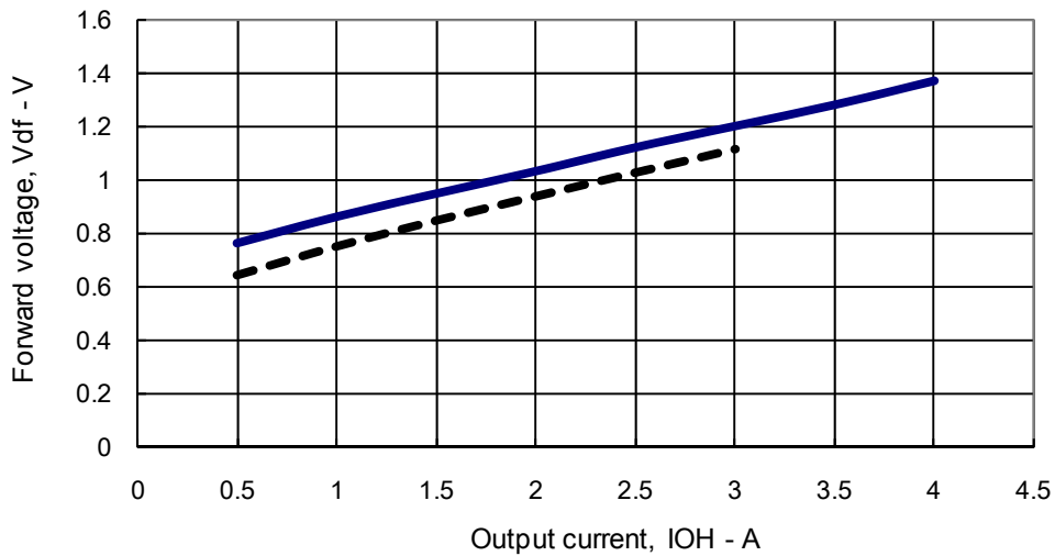
STK672-440BN. 442BN-E Forward voltage, V_{df} - Output current, I_{OH}
