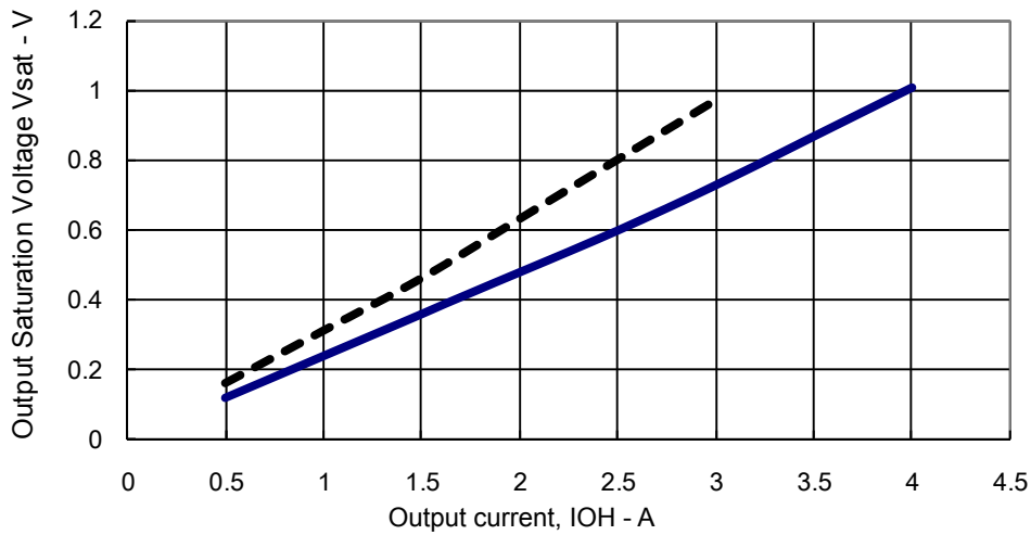
STK672-440BN. 442BN-E Output Saturation Voltage V_{sat} vs. Output Current
