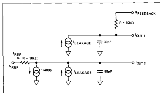
FIGURE 3: PM-7541A Equivalent Circuit (All Inputs LOW)
