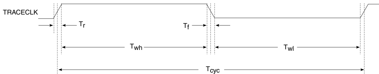
Figure 5. TRACE_CLKOUT specifications
