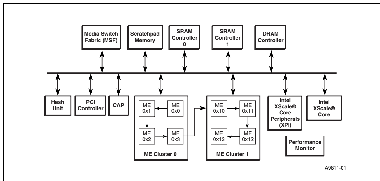
Figure 4. IXP2400 Network Processor Chassis Concept Block Diagram
