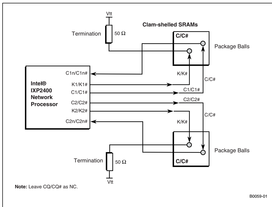
Figure 7. Clock Configuration
