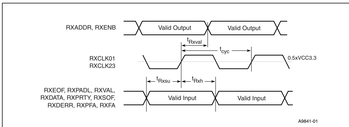
Figure 38. Receive UTOPIA/POS/CSIX
