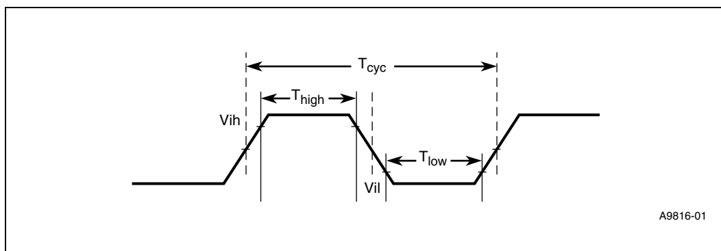
Figure 13. SYS_CLK Timing
