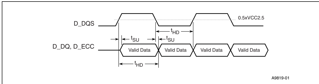
Figure 18. Data and Error Correction Setup/Hold Relationship to/from Data Strobe (Read Operation)
