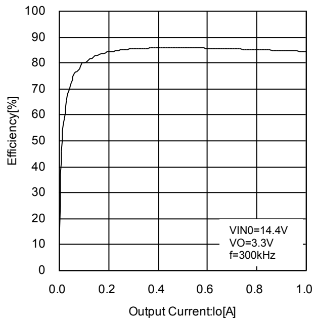
Figure 21. DCDC2 Conversion Efficiency vs Output Current
