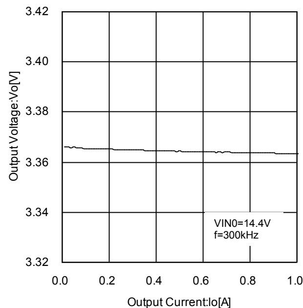
Figure 22. DCDC2 Output Voltage vs Output Current
