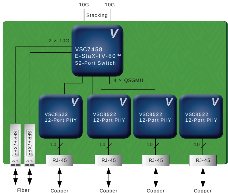
40 × 1 GbE + 4 × 10 GbE Stackable Managed Switch (Copper 1 GbE Ports)
