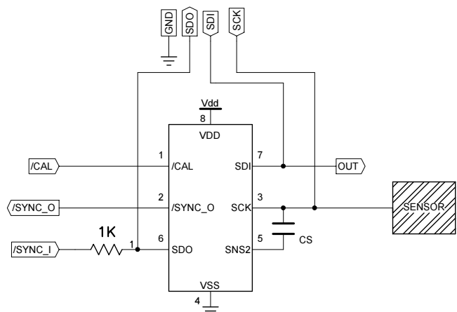
Figure 4-1 Clone interface wiring
