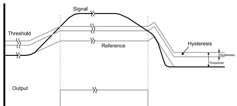
Figure 2-1 Drift Compensation
