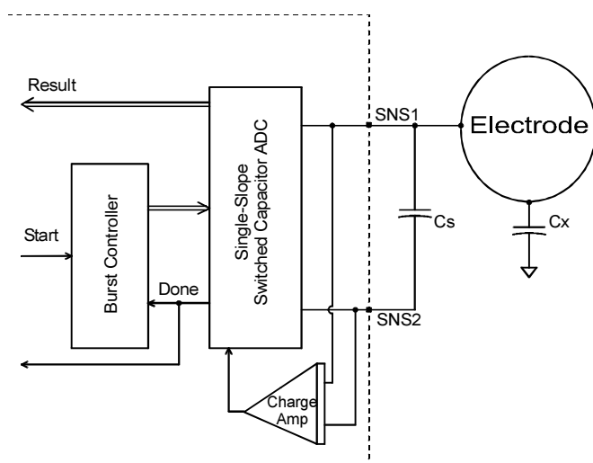
Figure 1-2 Internal Switching
