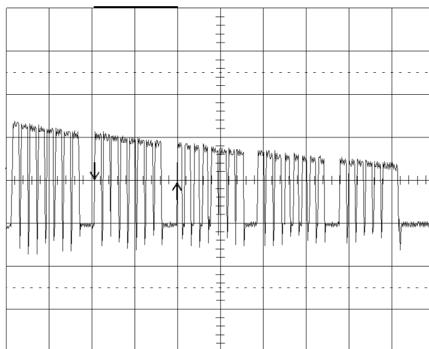
Figure 1-6 Burst Detail
