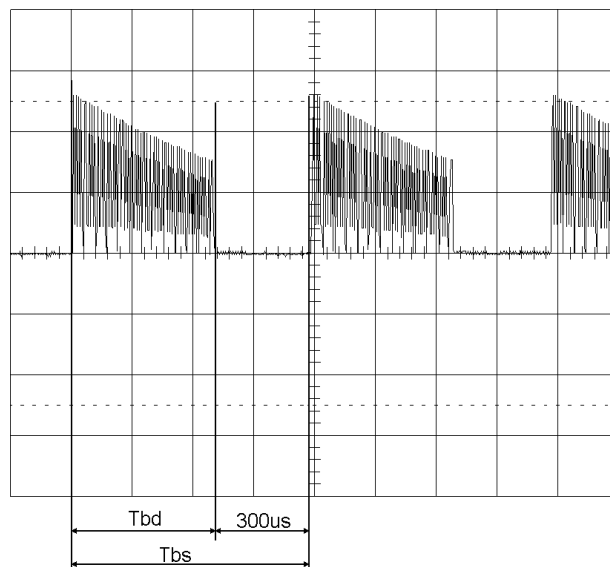
Figure 1-8 Burst when SC is set to 0 (no sleep cycles) (Observed using a 750K resistor in series with probe)
