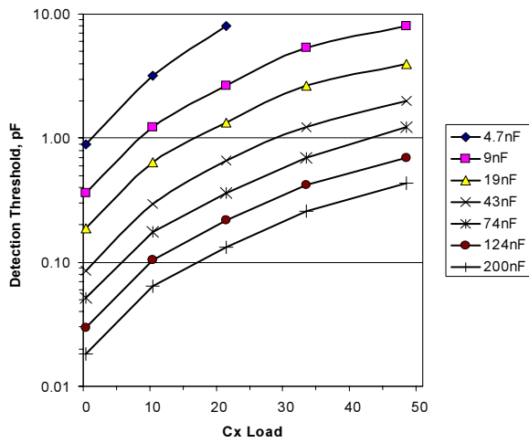
Figure 5-1 Typical sensitivity vs Cx; Threshold = 16, Vdd = 3.0 Volts
