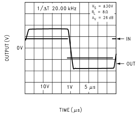
Pulse Response
