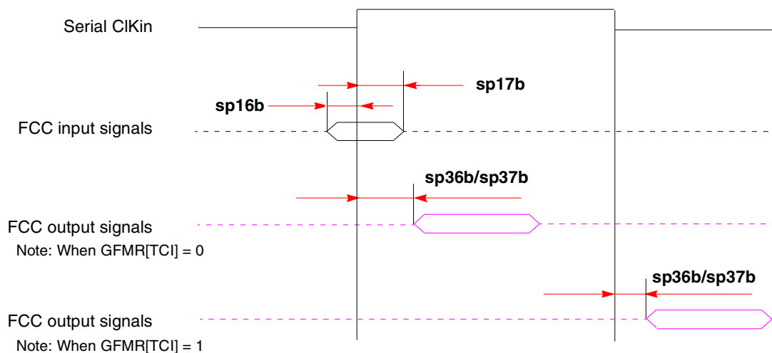
Figure 4. FCC External Clock Diagram
