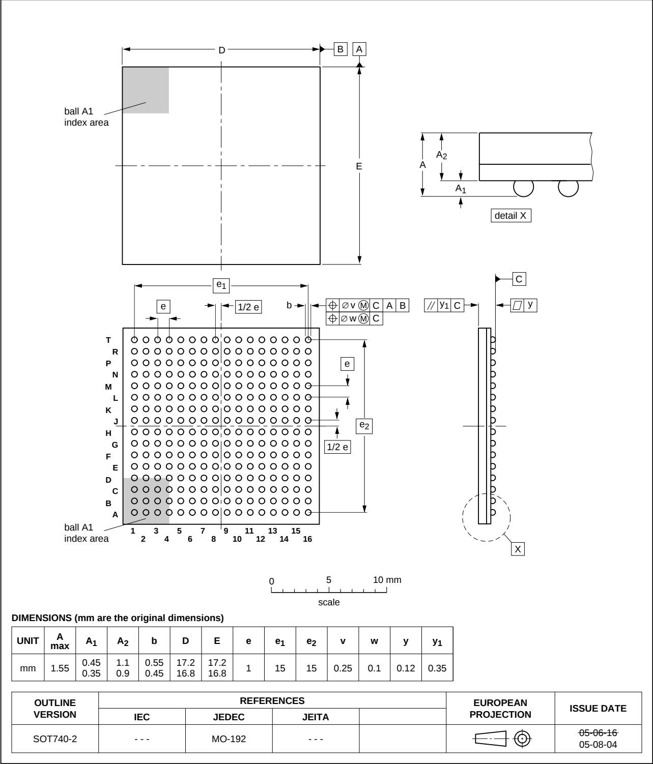
Fig 46. Package outline LBGA256 package
