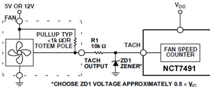
Figure 20. Fan with Strong TACH Pullup to >VCC or Totem-Pole Output, Clamped with Zener Diode and Resistor
