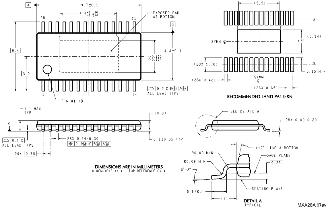
Molded TSSOP-28 NS Package Number MXA28A
