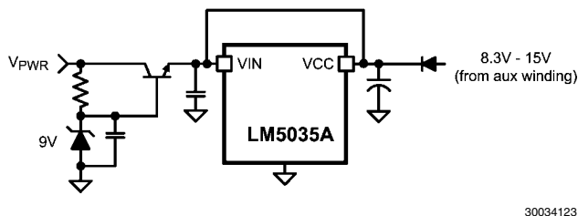
FIGURE 7. Start-up Regulator for V_{PWR} > 100V
