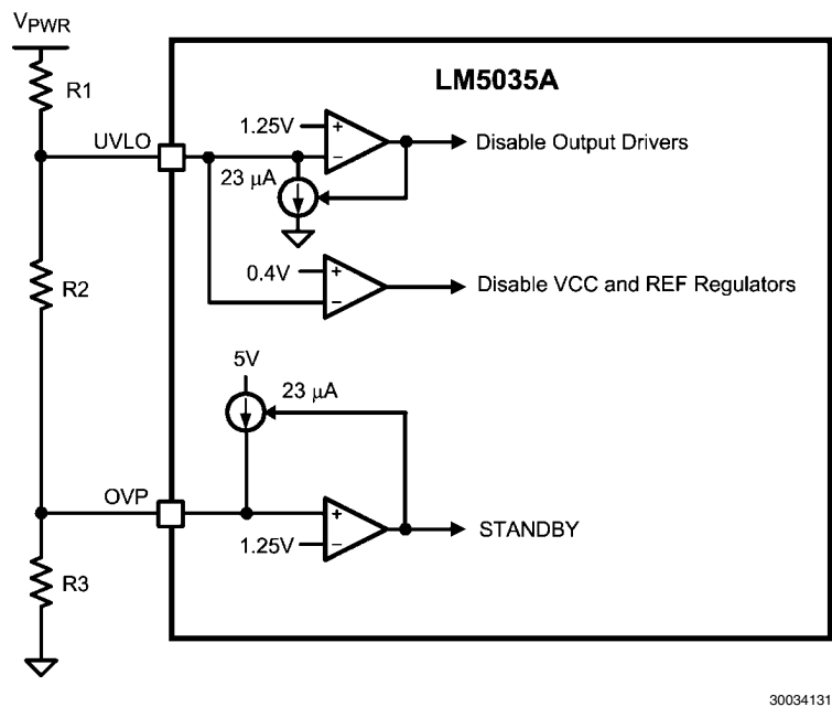
FIGURE 12. UVLO/OVP Divider
