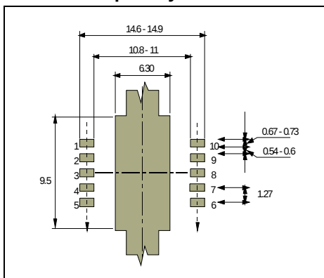
Figure 32. PowerSO-1 pad layout
