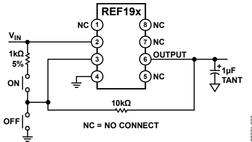
Figure 22. Membrane Switch-Controlled Power Supply
