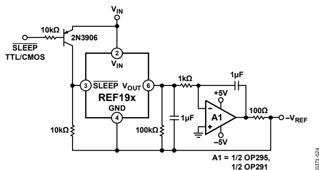
Figure 24. Negative Precision Voltage Reference Uses No Precision Resistors
