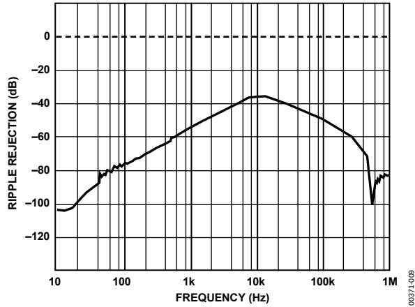
Figure 9. Ripple Rejection vs. Frequency
