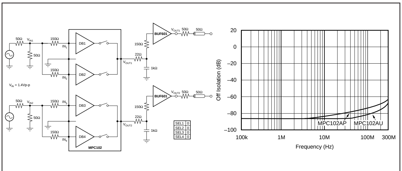
FIGURE 5. Off Isolation Test Circuit 2.
