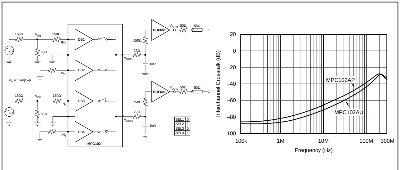
FIGURE 4. Off Isolation 150Ω Input.
