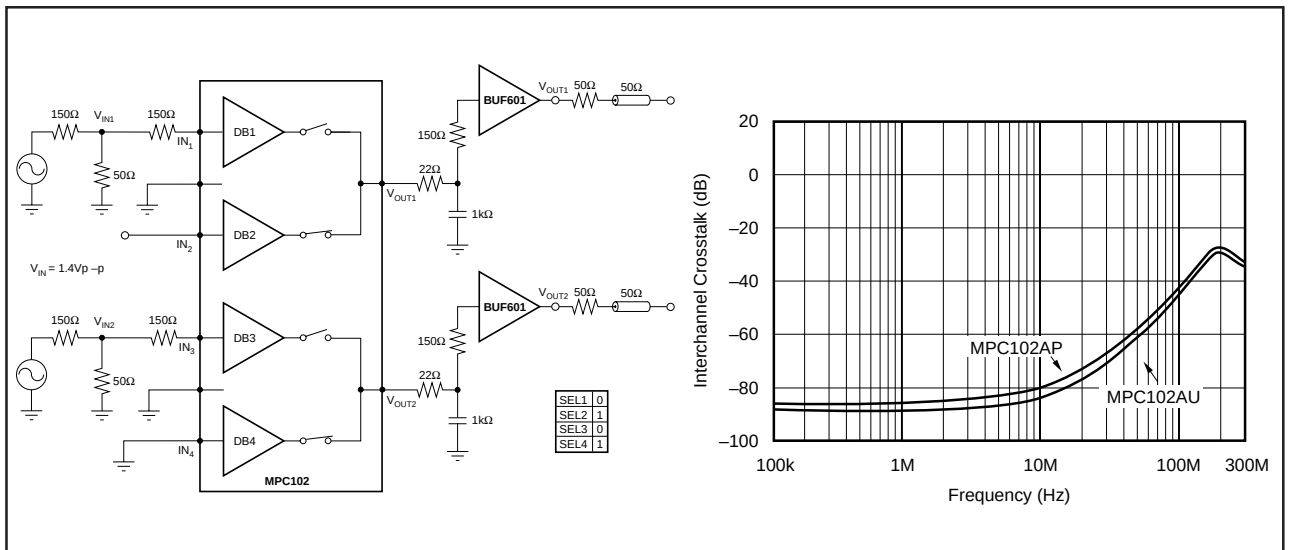
FIGURE 3. Channel Crosstalk – Grounded Input.
