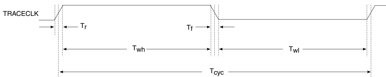
Figure 11. TRACE_CLKOUT specifications
