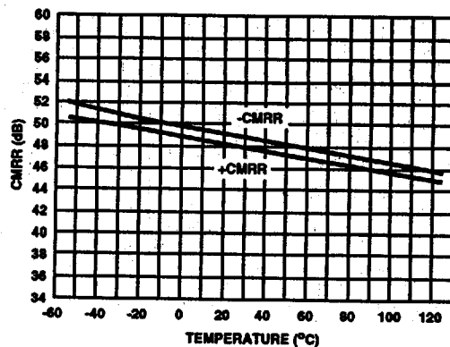
FIGURE 17. CMRR vs TEMPERATURE
