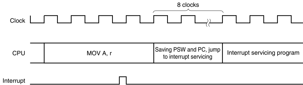
Figure 14-9. Interrupt Request Acknowledgement Timing (Example of MOV A, r)
