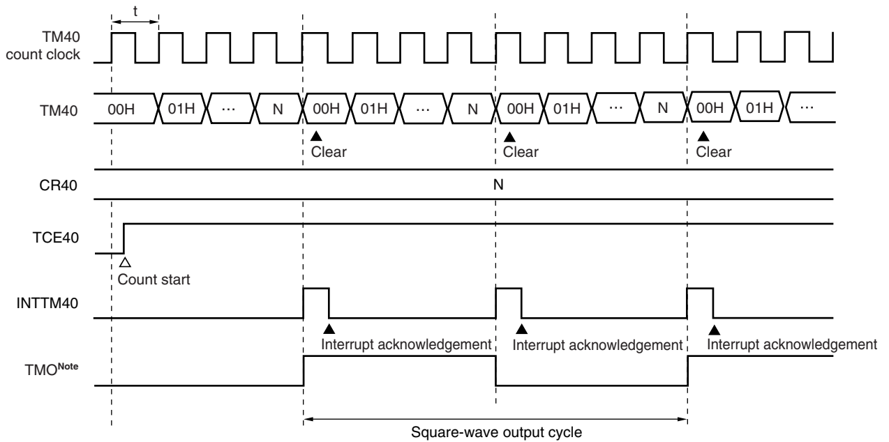
Figure 9-15. Timing of Square-Wave Output with 8-Bit Resolution
