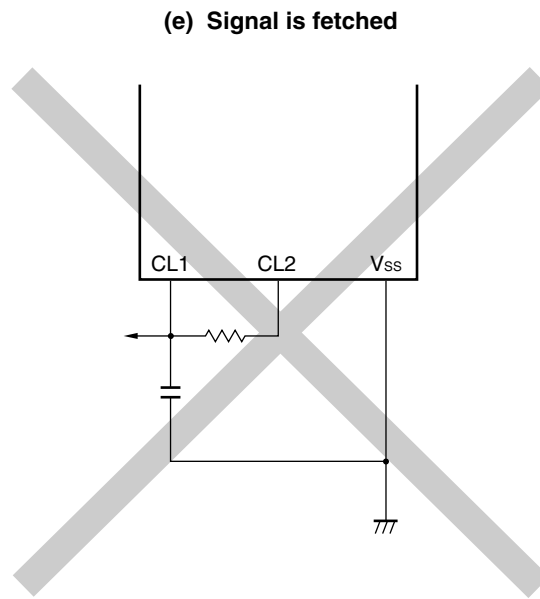
Figure 8-4. Example of Incorrect Resonator Connection (2/2)
