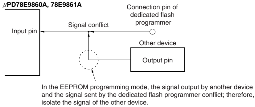
Figure 17-5. Signal Conflict (Input Pin of Serial Interface)
