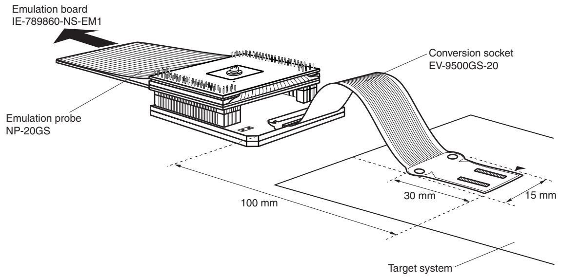
Figure B-2. Connection Conditions of Target System
