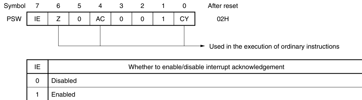
Figure 14-4. Program Status Word Configuration
