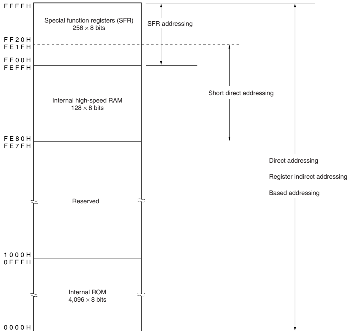
Figure 4-3. Data Memory Addressing ( \mu PD789052, 789062)
