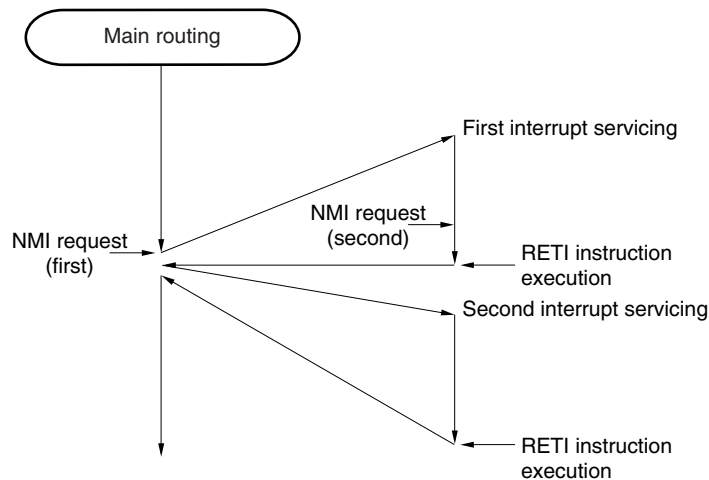
Figure 14-7. Acknowledgement of Non-Maskable Interrupt Request
