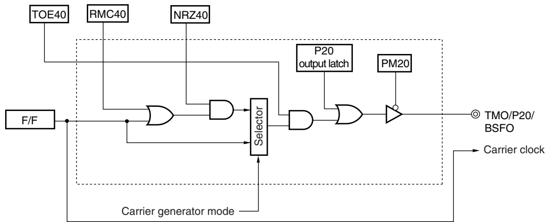
Figure 9-3. Block Diagram of Output Controller (Timer 40)
