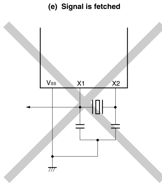
Figure 7-4. Example of Incorrect Resonator Connection (2/2)
