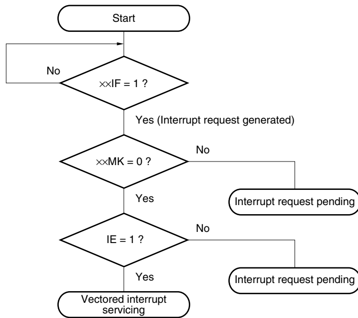
Figure 14-8. Interrupt Request Acknowledgement Processing Algorithm
