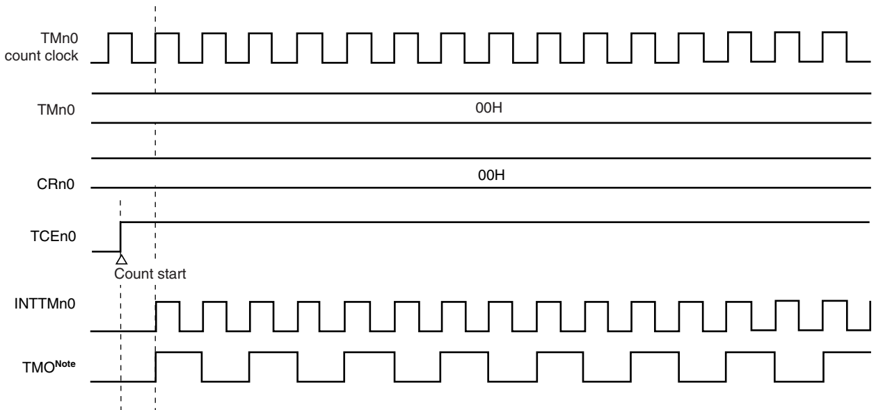
Figure 9-9. Timing of Interval Timer Operation with 8-Bit Resolution (When CRn0 Is Set to 00H)
