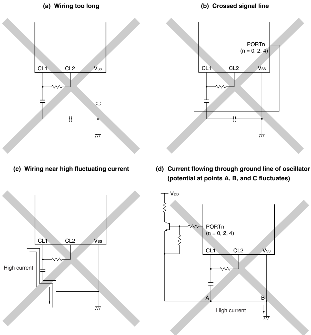
Figure 8-4. Example of Incorrect Resonator Connection (1/2)
