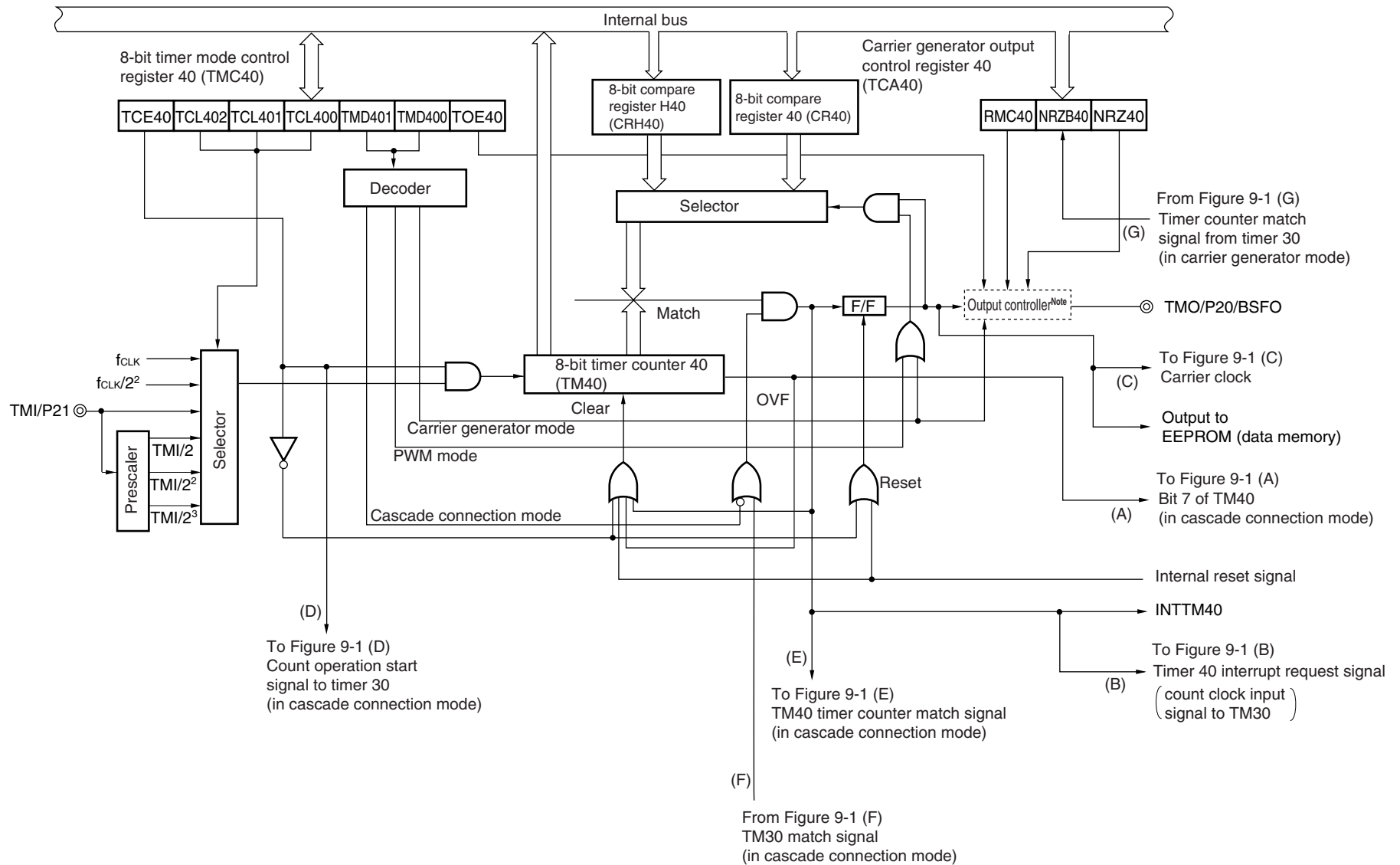
Figure 9-2. Timer 40 Block Diagram
