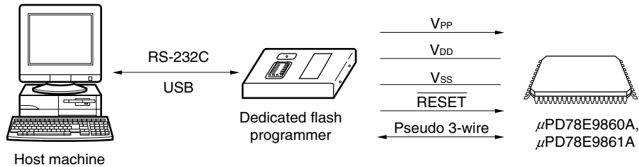
Figure 17-1. Environment for Writing Program to EEPROM (Program Memory)
