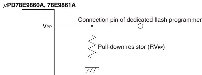
Figure 17-4. V PP Pin Connection Example
