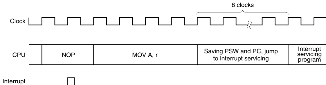
Figure 14-10. Interrupt Request Acknowledgement Timing (When Interrupt Request Flag Is Set at Last Clock During Instruction Execution)
