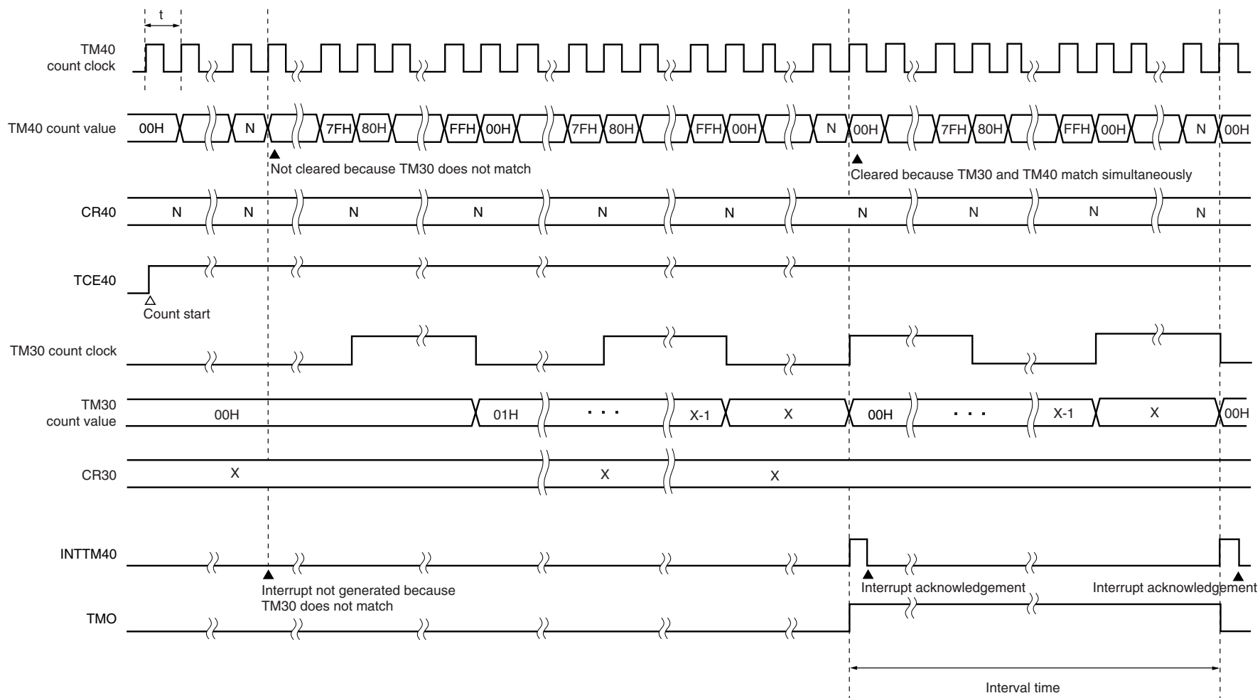
Figure 9-16. Timing of Interval Timer Operation with 16-Bit Resolution
