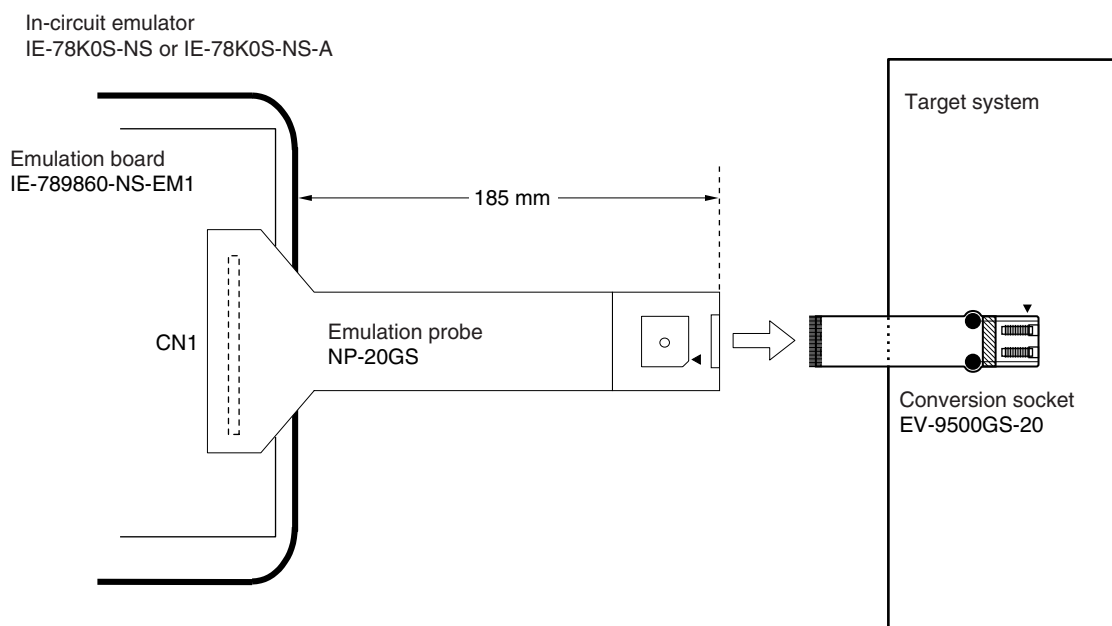
Figure B-1. Distance Between In-Circuit Emulator and Conversion Socket
