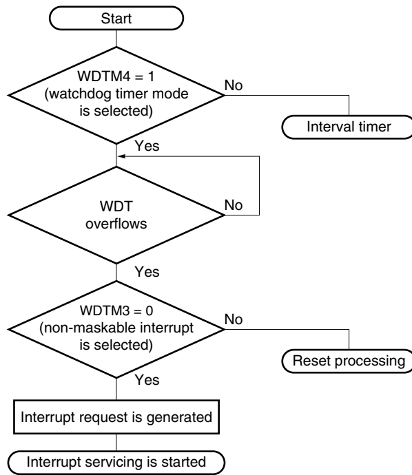
Figure 14-5. Flowchart from Non-Maskable Interrupt Request Generation to Acknowledgement (INTWDT)
