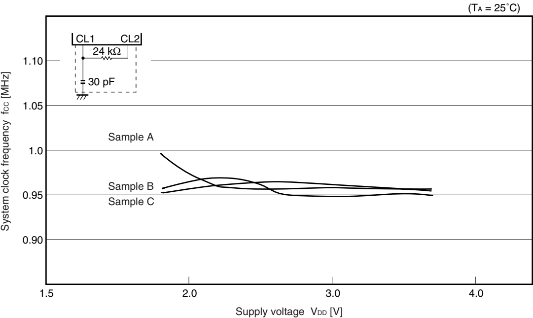
f_{cc} vs. V_{DD} (RC Oscillation: \mu PD789062, R = 24\text{ k}\Omega , C = 30\text{ pF} )
