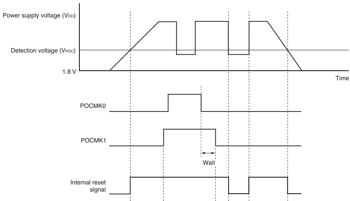
Figure 11-6. Timing of Internal Reset Signal Generation in POC Switching Circuit
