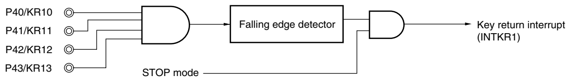
Figure 13-1. Block Diagram of Key Return Circuit
