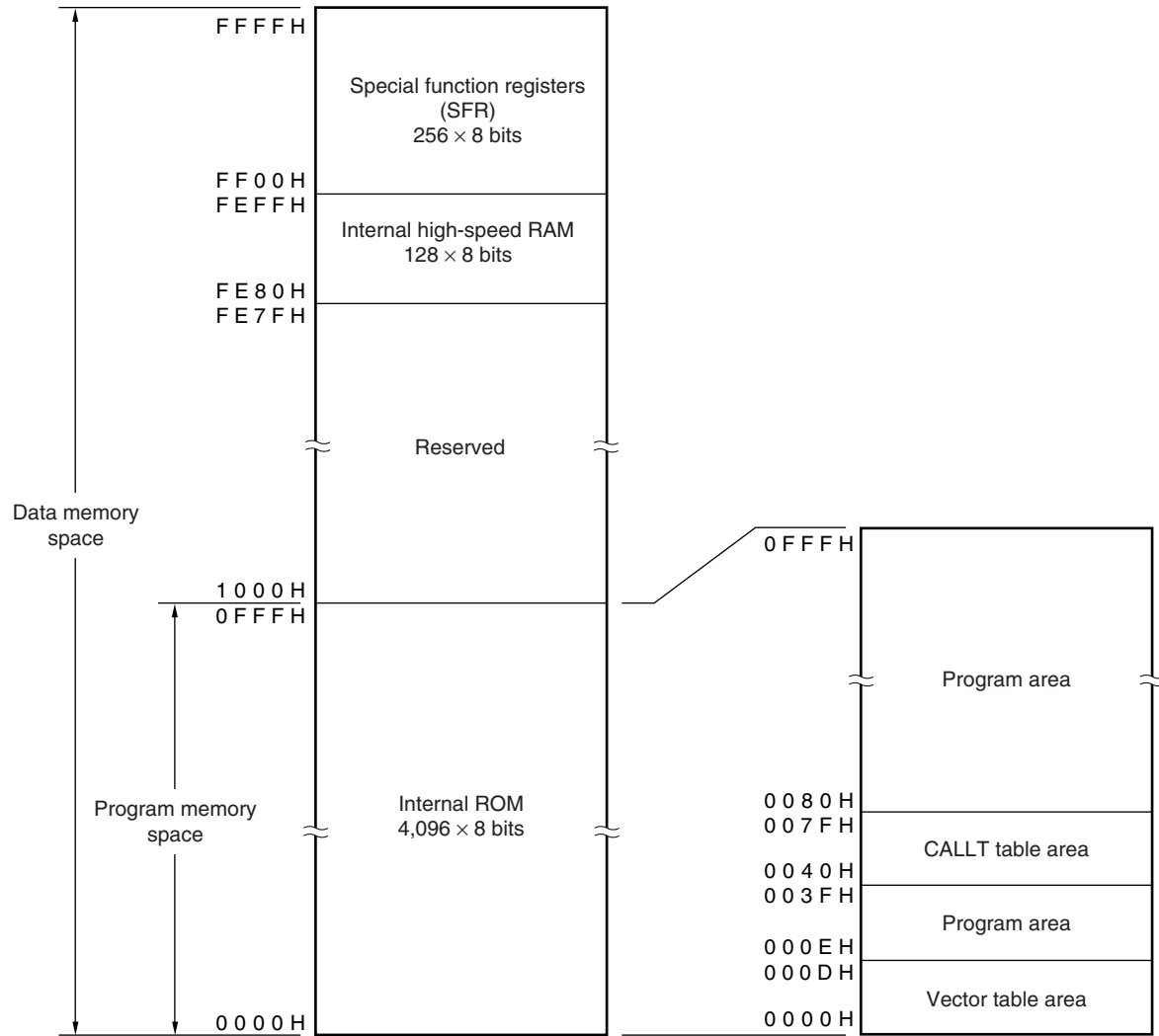
Figure 4-1. Memory Map ( \mu PD789052, 789062)
