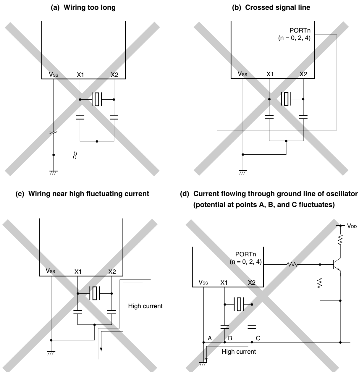
Figure 7-4. Example of Incorrect Resonator Connection (1/2)
