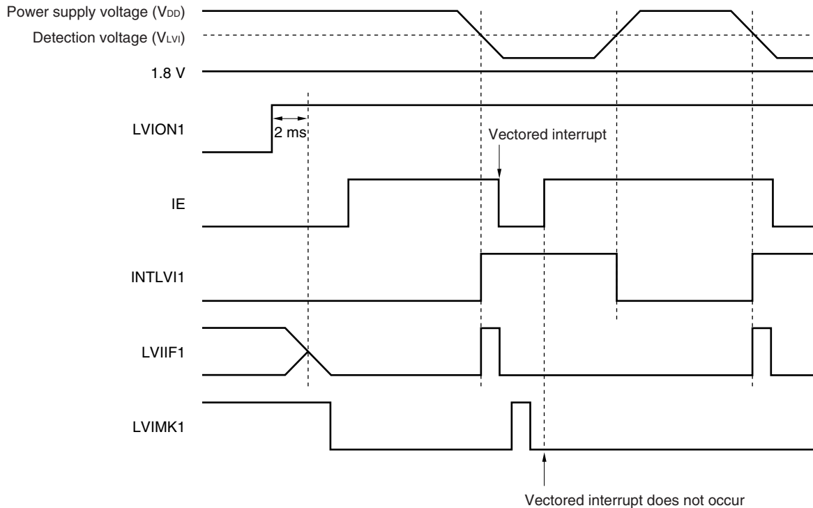
Figure 11-7. LVI Circuit Operation Timing
