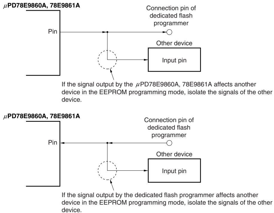
Figure 17-6. Abnormal Operation of Other Device
