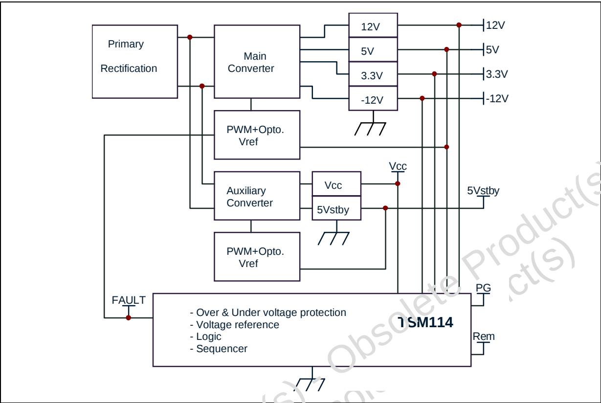
Figure 2: Internal Schematic
