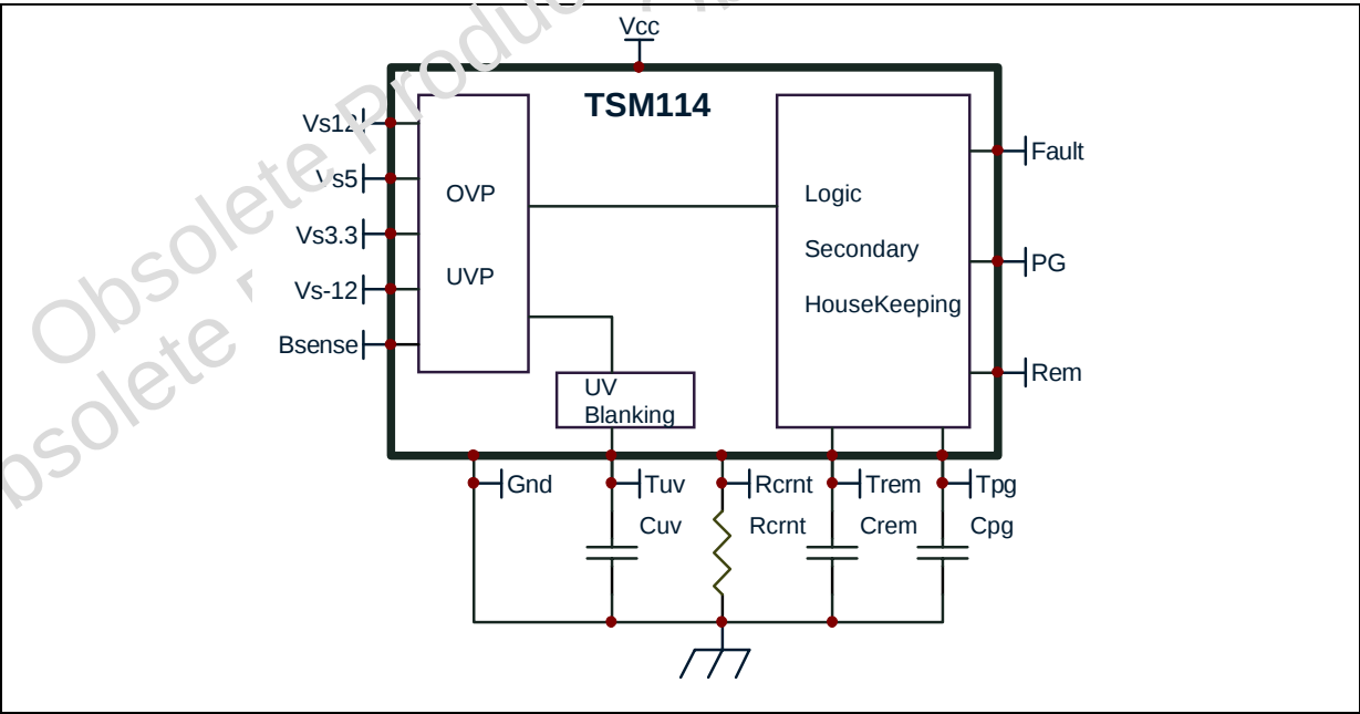
Figure 2: Internal Schematic
